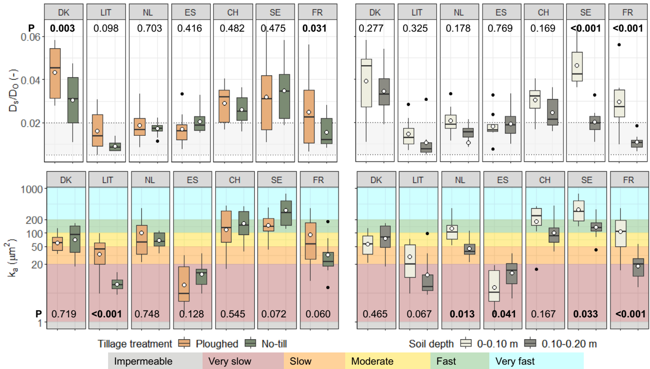
FIGURE 4 | Top: Relative gas diffusivity ( D_s/D_0 ) at -100 hPa matric potential by location and tillage practice (left) and soil depth (right). The marked area at D_s/D_0 = 0.005-0.020 reflects the critical range for oxic soil conditions (e.g., Schjønning et al. 2003). Bottom: Darcian air permeability ( k_a ) at -100 hPa matric potential by location and tillage practice (left) and soil depth (right). The coloured background indicates the classification of air permeability following Fish and Koppi (1994) and Ball et al. (1988). The boxplots display the median (central line), interquartile range (IQR, box), and whiskers (indicating data points within 1.5 times the IQR). Black points outside the whiskers represent potential outliers. ● = estimated mean; p -values are given per site.
