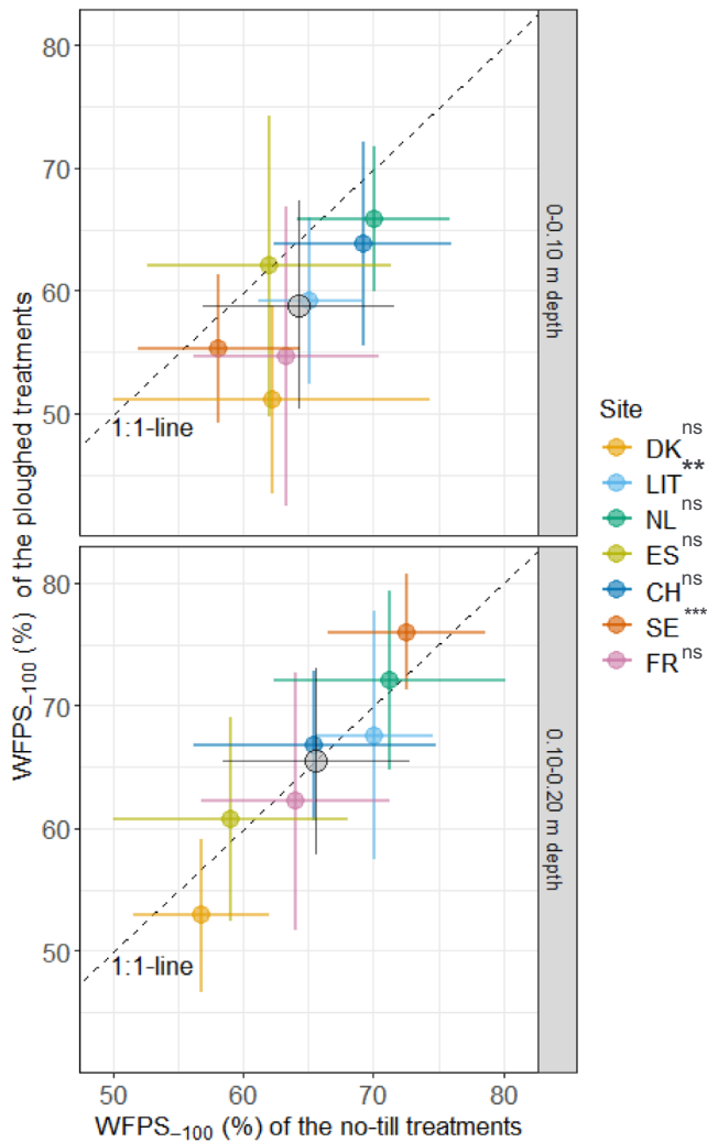
FIGURE 2 | Water-filled pore space at -100 hPa matric potential ( WFPS_{-100} ) at different locations and soil depths for ploughed and no-till treatments (mean and standard deviation, n=4 ). ● = mean across the locations ( p=0.004 for the interaction of treatment and depth). Significant differences between soil depths for a given location are indicated in the legend with: *** \leq 0.001 ; ** \leq 0.01 ; ns \geq 0.05 .
