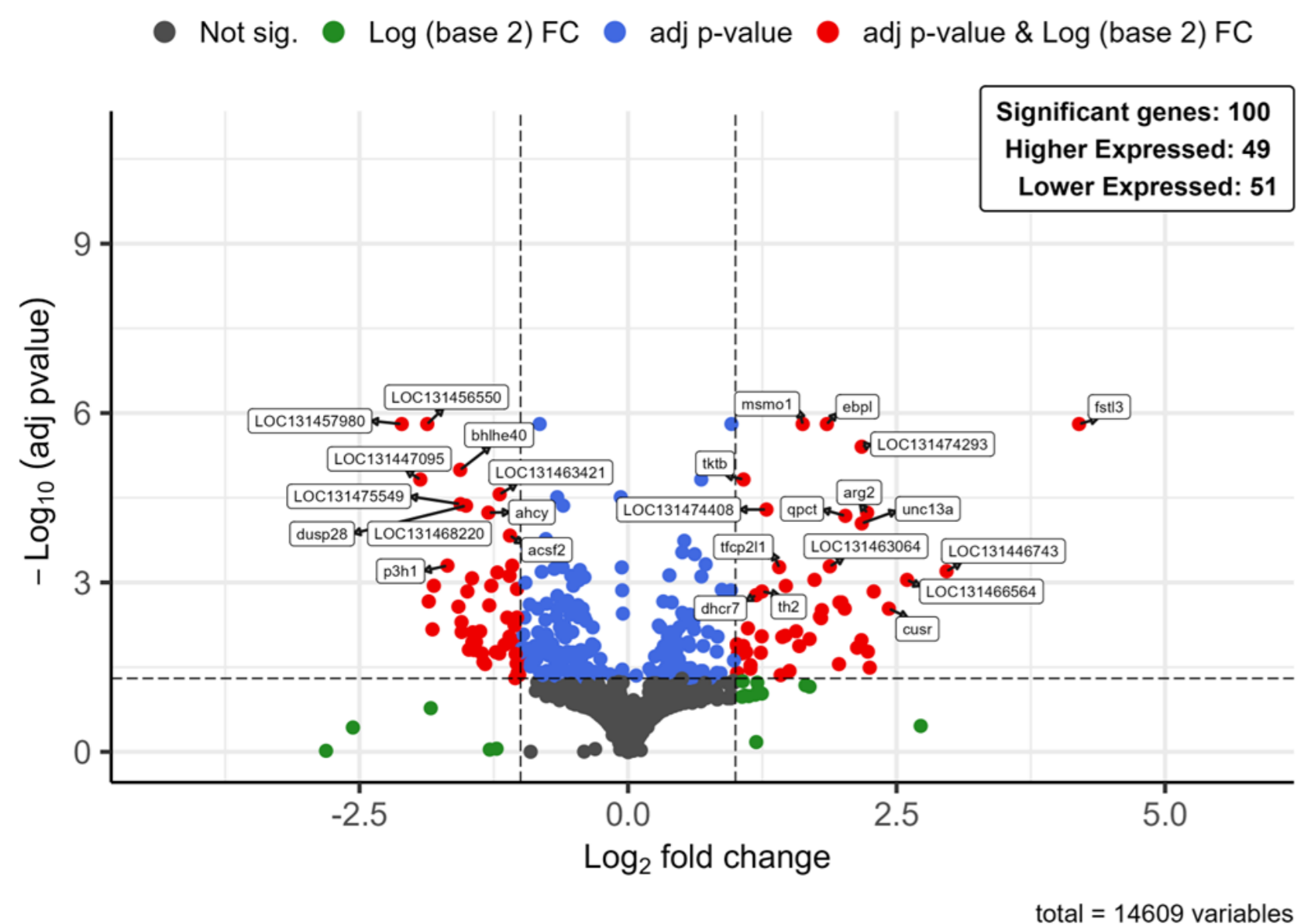
Development of a bio-assay (RNAseq)
