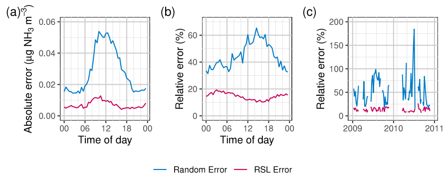
Fig. A.1. Mean diurnal variation of (a) absolute error and (b) relative error for (blue) random error and (red) error due to RSL. (c) Weekly average random error and error due to RSL.
