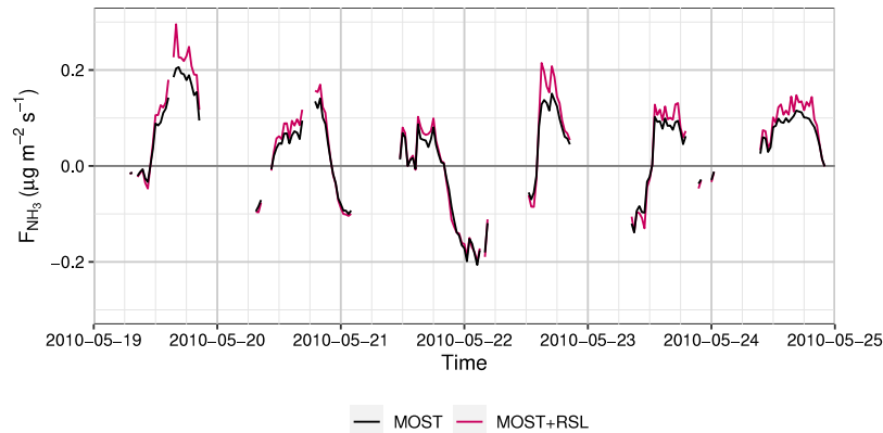
Fig. A.4. F_{\text{NH}_3} for 6 days in May 2010, calculated with both MOST and MOST+RSL.
