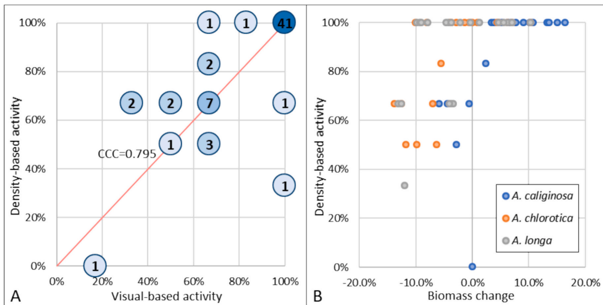
Fig. 1. (A) Relation between visual-based and density-based earthworm activity for the species for which estimation rate could be investigated ( A. chlorotica , A. caliginosa and A. longa ). Numbers in dots (as well as the intensity of dot-colour) represent the amount of overlapping observations. CCC = concordance correlation coefficient. (B) Relation between earthworm biomass change and density-based activity for the same three earthworm species.
