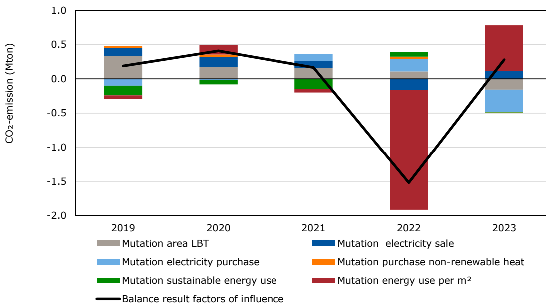
Figure S.3 Effects of emission boosting (+) and emission damping (-) factors of influence after temperature correction by year for 2019 - 2023 (Mton) v) v) Results for 2023 are provisional.
