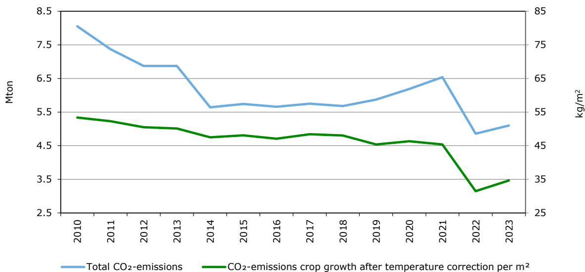
Figure S.2e Total CO 2 emissions and CO 2 emissions for crop growth per m 2 after temperature correction of Dutch greenhouse horticulture per year 2010-2023 v) v) Results for 2023 are provisional.
