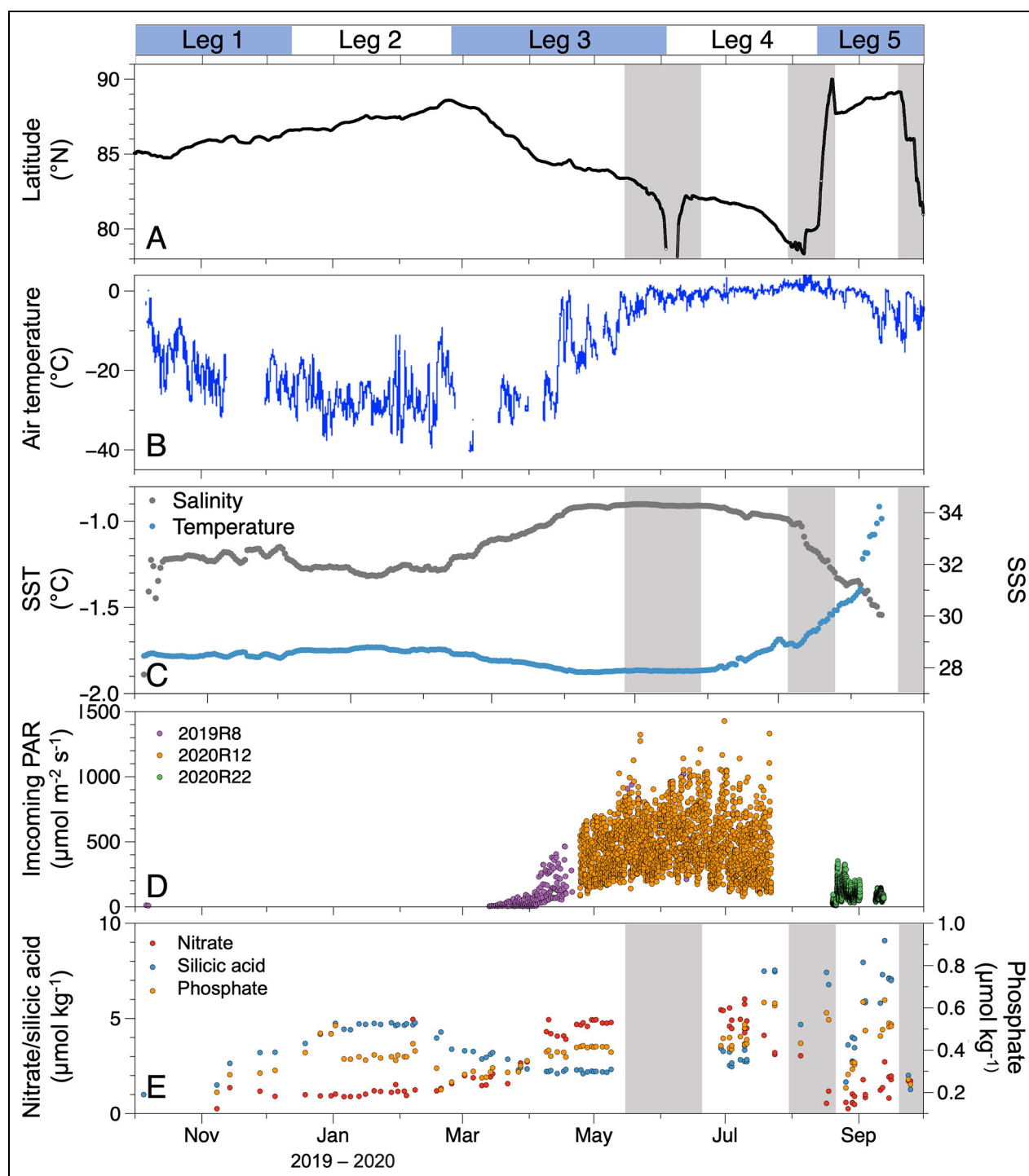
Figure 9. Environmental conditions over the annual cycle of the drift year. (A) Latitude ( ^{\circ} N), (B) air temperature at 2 m height, (C) sea surface temperature (SST, blue) and salinity (SSS, gray) at 10 m depth, (D) incoming photosynthetically active radiation (PAR; 400–700 nm, measured as photon flux density) from three different radiation stations on the MOSAiC floes (and CO 3 ; 2019R8 in pink in CO 1 , 2020R12 in orange in CO 1 and CO 2 , and 2020R22 in green in CO 3 ), and (E) surface ocean nutrients (nitrate + nitrite, silicic acid, and phosphate) from all samples collected from the upper 30 m of the water column. Gray-shaded areas indicate transit periods. Here, latitude and nutrients are from the location of RV Polarstern , while surface air temperature, water temperature, and PAR are representative of the respective central observatory conditions.
