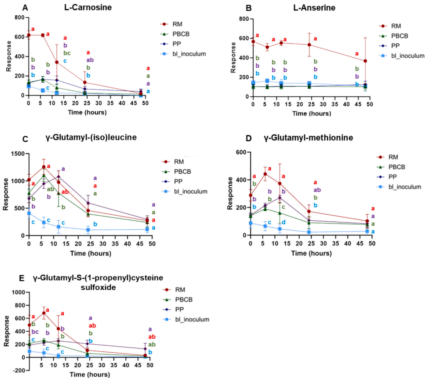
Fig. 6. Response of (A) L-carnosine (B) L-anserine, (C) gamma-glutamyl-(iso)leucine, (D) gamma-glutamyl-methionine, and (E) gamma-glutamyl-S-(1-propenyl) cysteine sulfoxide. Notes: RM beef patty, PBCB plant-based commercial patty, PP plant-based homemade patty, bl_inoculum, sample without any substrate. The different letters indicated the significant difference by two-way ANOVA analysis for different groups at the same time point.
