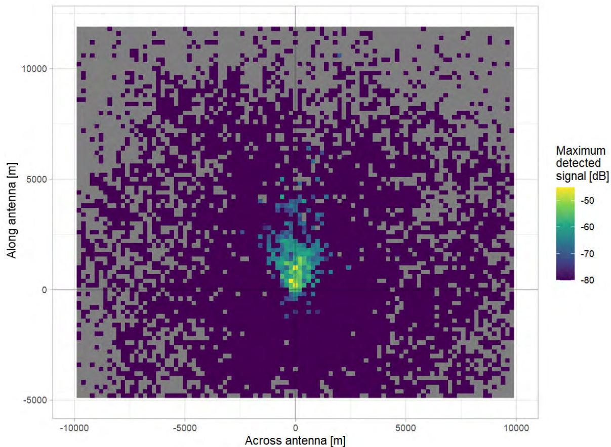
Figure A13-2: Simultaneous GPS and MOTUS detections rotated in the direction of the receiving MOTUS antenna. The data is grided and only the maximum detected MOTUS signal is displayed for each cell (200[m] x 200[m]). This illustration also shows 'null' detections (where there is a GPS location fix but no MOTUS detection) as -80 [dB] (dark blue). Areas with no MOTUS detections and GPS location fixes are shown as grey.
