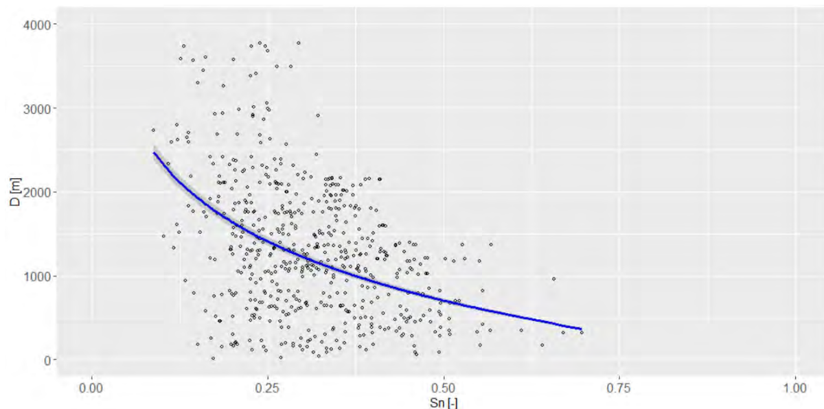
Figure A13-3: predictor effect plot of the relation between normalized signal strength (Sn) and distance from the receiver in the direction of the antenna (D). The dots represent the measurements.
