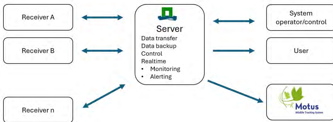
Figure 7: Schematic overview of added functionality WUR server
