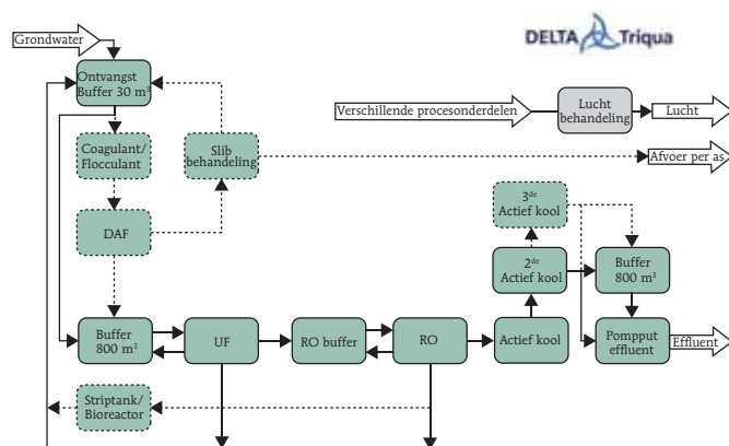
FIGUUR 5: FLOWSHEMA WATERZUIVERING.
