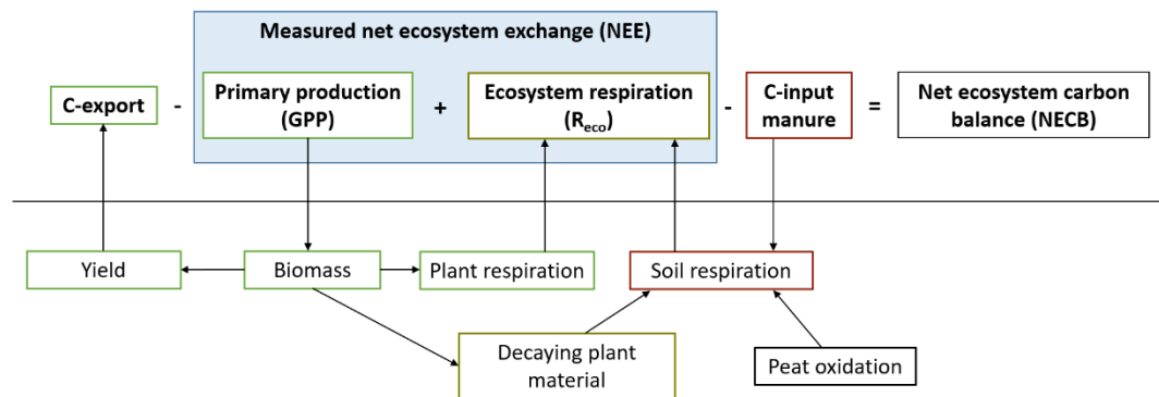
Figure 1 Simplified schematic overview of the components that contribute to the different measured and partitioned carbon fluxes (C-export, GPP and R_{eco} ), which sums up to the NECB. Soil respiration consists of both young, plant and manure derived carbon, and old (fossil), peat derived carbon.
