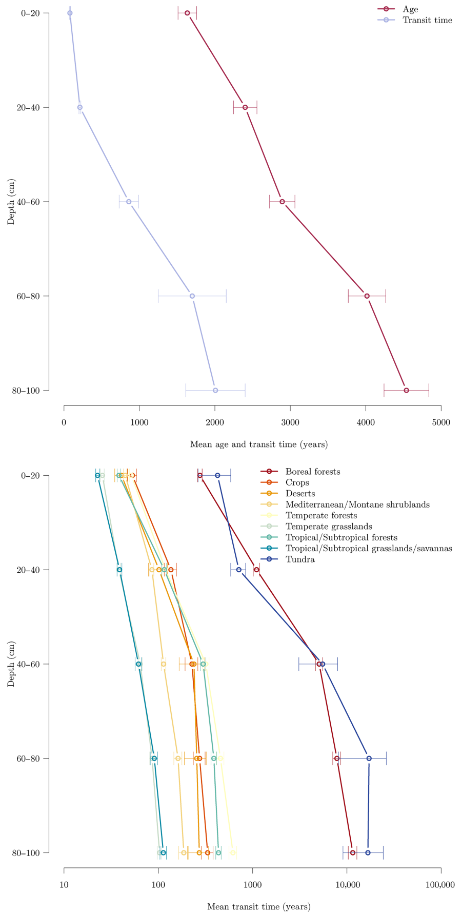
FIGURE 8 Estimates of mean age and mean transit time of carbon based on measurements of root inputs and soil radiocarbon obtained from ISRaD. The upper panel shows global-scale average values of mean age and mean transit time. The lower panel shows averages of mean transit time aggregated by biome.
