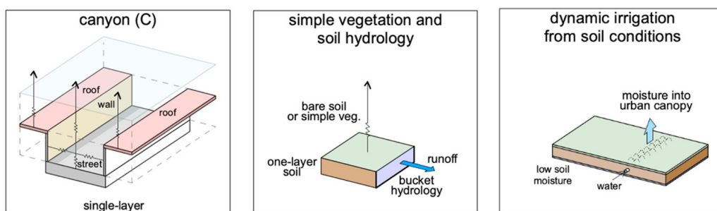
FIGURE A13 K-UCMv1 (Klimaat Urban Canopy Model v1) solves the local surface energy balance based on land cover input and regional meteorological forcing. To calculate conduction, the urban facets (ground, roof, walls) have 10 layers. Effects of low vegetation are accounted for in the surface energy balance without shadowing effects. Vegetation is perfectly watered and non-vegetation surfaces store no water. [Colour figure can be viewed at wileyonlinelibrary.com ]
