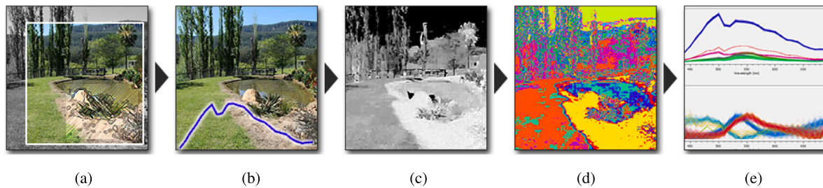
Fig. 8. Shows the processing pipeline of a hyperspectral image using AI tools: (a) represents the pre-processing, (b) represents the illumination recovery, (c) represents the reflectance recovery, (d) represents the area clustering, and (e) analysis the different statistical values of the hyperspectral image in the form of a graph (Habibi & Oorloff, 2015).
