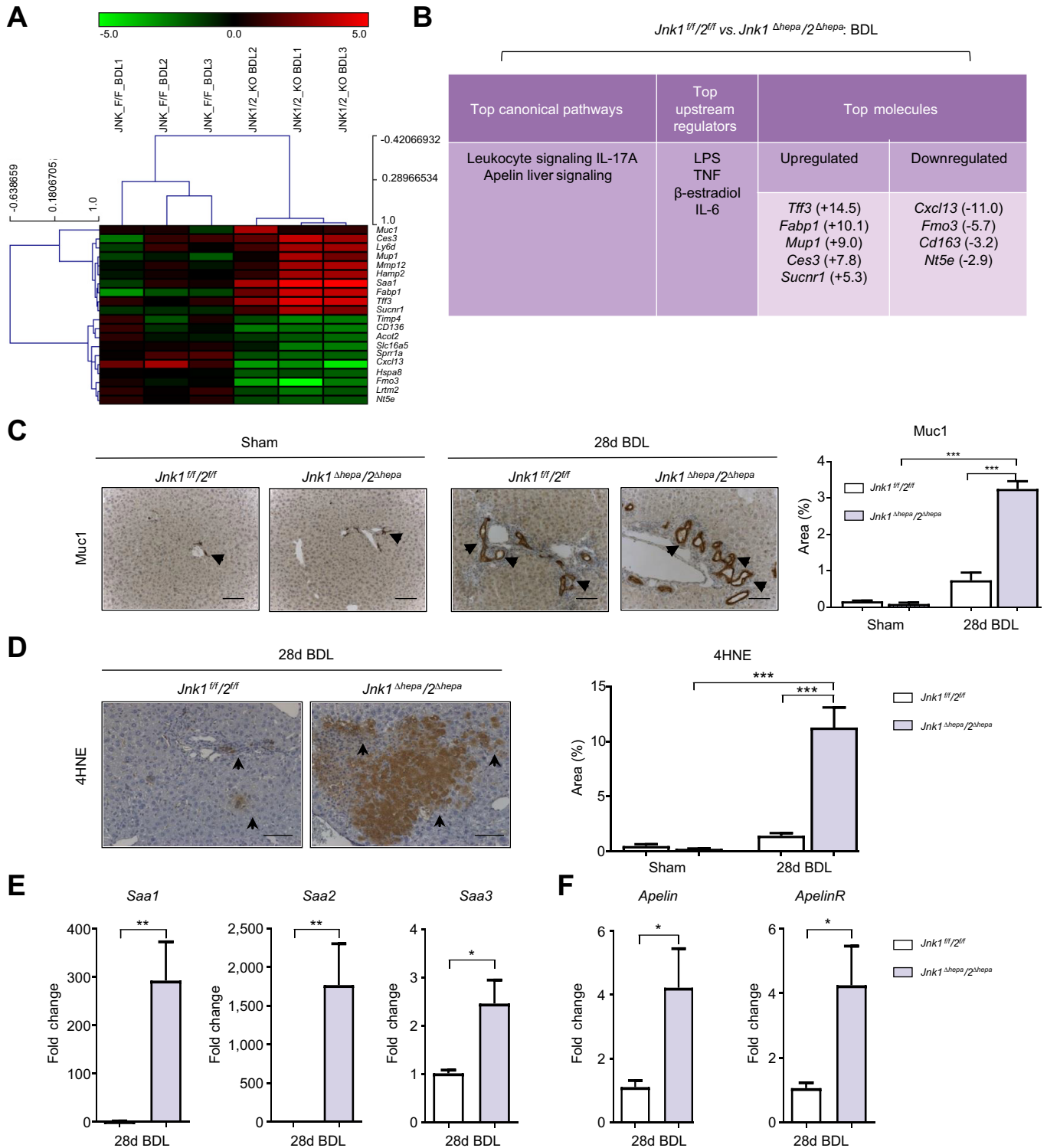
Fig. 5. Jnk1/2 -dependent pathways during BDL-induced cholestatic liver injury. (A) Gene array analysis was performed in Jnk1 fl/fl and Jnk1 Δhepa/2 Δhepa livers, 28 days after BDL. Log 2 expression values of the individual mice were divided by the mean of the sham-operated mice. Log ratios were saved in a .txt file and analysed using the Multiple Experiment Viewer. Heat map of the top-regulated, upregulated, and downregulated genes (red, upregulated; green, downregulated, n = 3, -5.0 <fold change >5.0). (B) Ingenuity Pathway Analysis was performed in the same liver samples. The top canonical pathways (left panel), the top upstream regulators (middle panel), and the top up- and down-regulated genes (right panel) are represented. (C, D) Representative immunohistochemistry staining for Muc1 and 4HNE of paraffin sections from Jnk1 fl/fl and Jnk1 Δhepa/2 Δhepa livers (n = 5), 28 days after BDL. Scale bar = 100 μm. The positive area percentage was quantified using Image J® software. Arrows indicate positive cells. (E, F) mRNA expression analysis of acute-phase response genes ( Saa1 , Saa2 , and Saa3 ), Apelin , and ApelinR was quantified by quantitative reverse-transcription PCR. Statistical evaluation was carried out by multicomparison one-way ANOVA followed by post hoc Bonferroni's test among three or more groups. Comparisons of two groups were analysed using an unpaired, two-tailed Student t test. Values are represented as mean ± SEM from five to six mice per group (n, not significant; *p <0.05; **p <0.01; ***p <0.001). 4HNE, 4-hydroxynonal; ApelinR, Apelin receptor; BDL, bile duct ligation; JNK, c-Jun-N-terminal kinase; LPS, lipopolysaccharide; Muc1, mucin 1; TNF, tumour necrosis factor.
