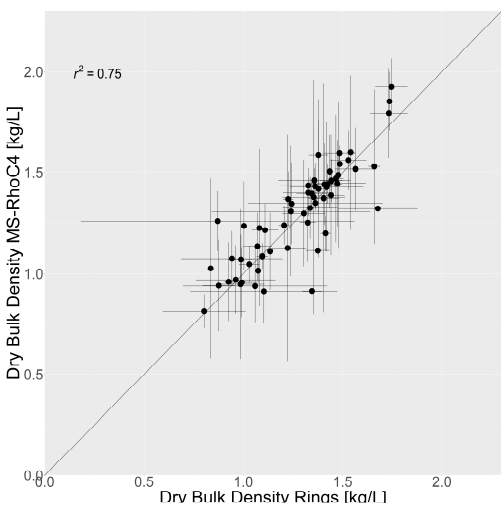
Figure 1. Dry bulk density averages per depth per location of sensor and ring (reference) data. Error bars are 2 times the standard deviation.
