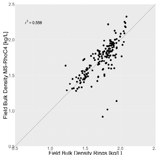
Figure 2. Field bulk density measurements with sensor and rings, not averaged per depth
