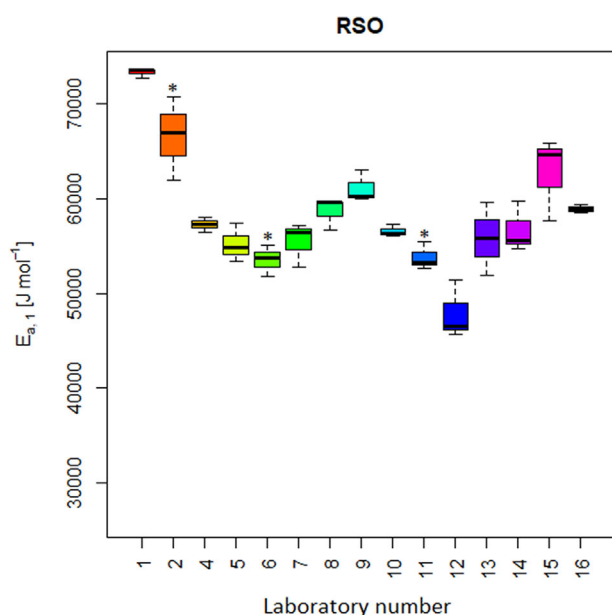
FIGURE 4 Activation energy ( E_{a,1} ; J mol -1 ) for RSO during storage at different temperatures (20°C, 30°C, 40°C, and 60°C) in 15 out of 16 different laboratories (anonymized and numbered from 1 to 16). Laboratory 3 was not included in the calculations. In the laboratories 2, 5, 6, 7, 9, and 11, the samples were frozen until analysis. Marked with an asterisk are laboratories 2, 6, and 11 that differ significantly ( p \leq 0.05 ) from the remaining laboratories that analyzed the samples directly after sampling.
