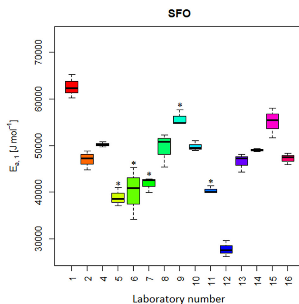
FIGURE 5 Activation energy ( E_{a,1} ; J mol -1 ) for SFO during storage at different temperatures (20°C, 30°C, 40°C, and 60°C) in 15 out of 16 different laboratories (anonymized and numbered from 1 to 16). Laboratory 3 was not included in the calculations. In the laboratories 2, 5, 6, 7, 9, and 11, the samples were frozen until analysis. Marked with an asterisk are laboratories 5, 6, 7, 9, and 11 that differ significantly ( p \leq 0.05 ) from the remaining laboratories that analyzed the samples directly after sampling.
