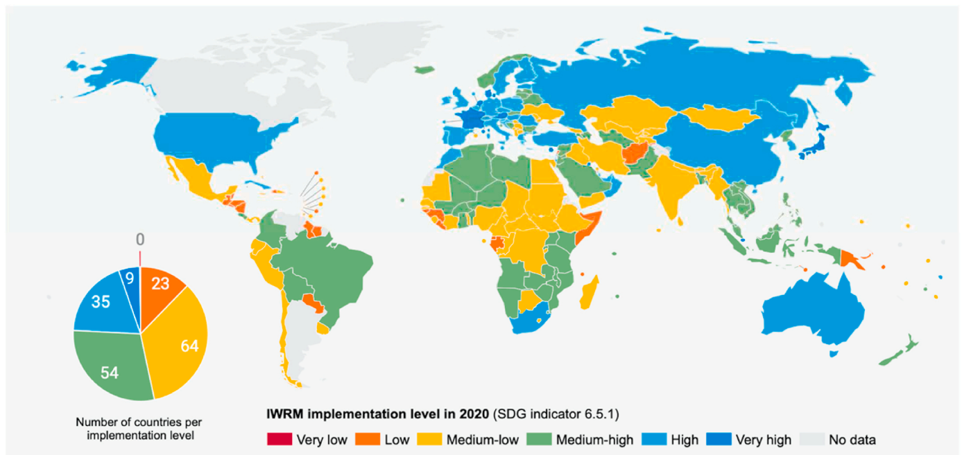
Fig. 2. IWRM implementation level in 2020. Source UNEP (2021).
