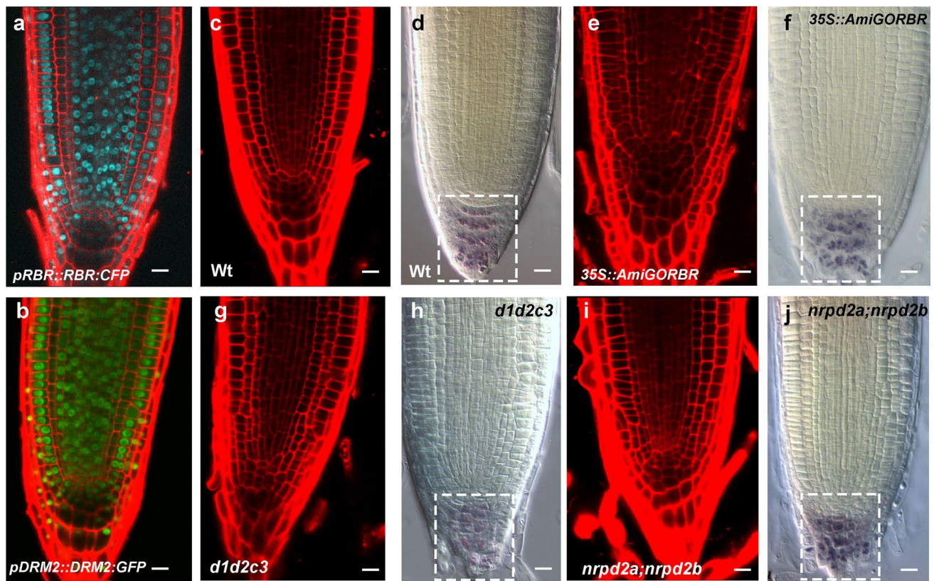
Fig. 3 Longitudinal root sections of 10 dpg seedlings imaged by confocal laser scanning microscope (CLSM) a–i and Nomarski optics of lugol-stained roots d, f, h and j . Panels a and b show the expression patterns of pRBR::RBR:CFP and pDRM2::DRM2:GFP . c confocal and d Nomarski optics images showing root apical meristem (RAM) and root stem cell niche (RSCN) organization in Col-0 (WT) seedlings. e Confocal and f Nomarski images of 35S::AmiGO-RBR seedlings showing alterations in the RAM and RSCN. g Confocal and h Nomarski images of drm1;drm2;cmt3 ( d1d2c3 ) triple mutant seedlings showing alterations in the RAM and the RSCN. i Confocal and j Nomarski images of nrpd2a;nrpd2b double mutant seedlings showing phenotypes in the RAM and RSCN, dotted squares highlight the Columella region. Bars in all panels = 50 μm
