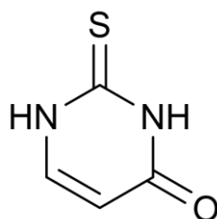
Figure 3.1. 2-Thiouracil chemical structure. Molecular weight: 128.15 \text{g mol}^{-1} , Molecular formula: \text{C}_4\text{H}_4\text{N}_2\text{OS}
