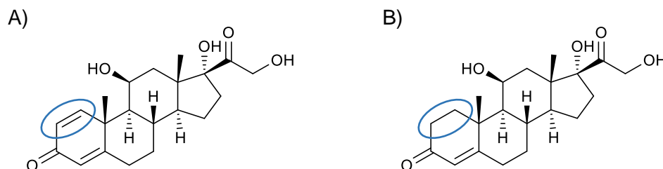
Figure 8.1. Molecular structures of (A) prednisolone and (B) cortisol.
