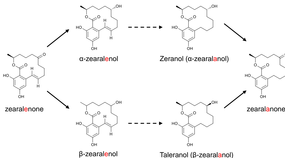
Figure 7.1. Overview of the metabolism of RALs, dashed arrows represent the conversion of the toxins towards zeranol.
