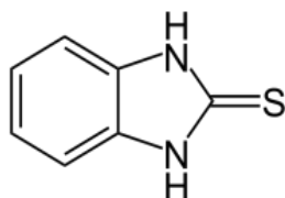
Figure 3.8. Molecular structure of 2-Mercaptobenzimidazol.
