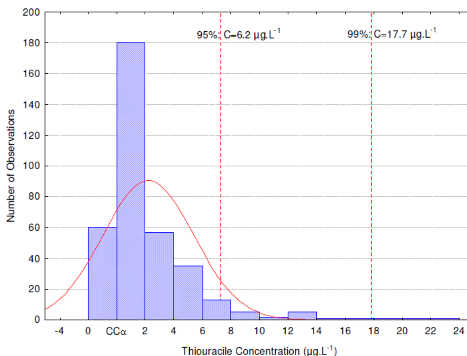
Figure 3.4. Frequency distribution of thiouracil in calf urine samples. Reproduced from [50].
