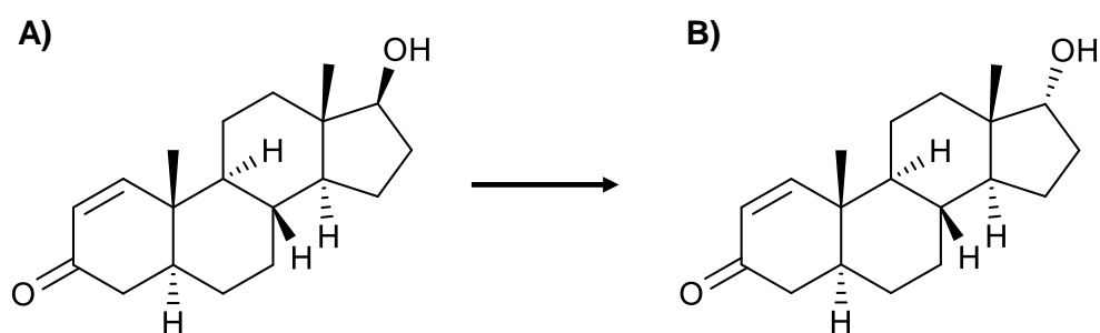
Figure 6.2. Metabolism of 1-testosterone (17 \beta -hydroxy-5 \alpha -androst-1-en-3-one) (A), main metabolite 17 \alpha -1-testosterone (17 \alpha -hydroxy-5 \alpha -androst-1-en-3-one) (B).
