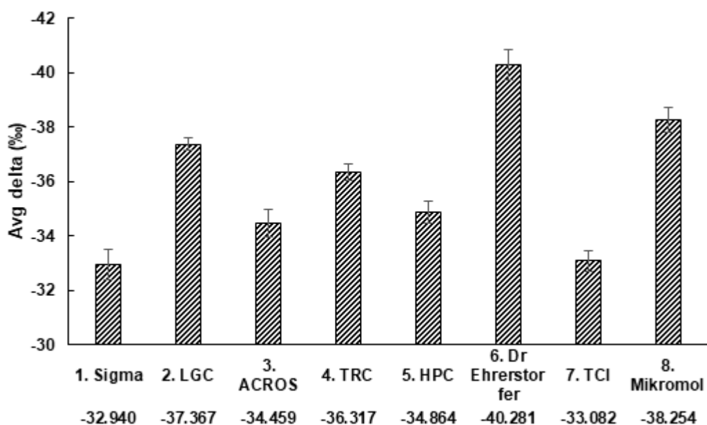
Figure 3.2 Carbon Isotope Ratio ( ^{13}\text{C}/^{12}\text{C} ) of 2-thiouracil standards of 8 different suppliers. The lower row is the average delta value.
