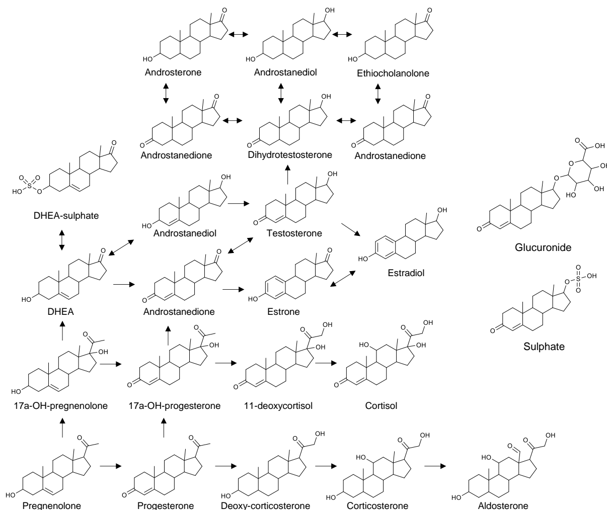
Figure 2.1. Steroidogenesis, the steroid pathway showing relations between individual steroids.
