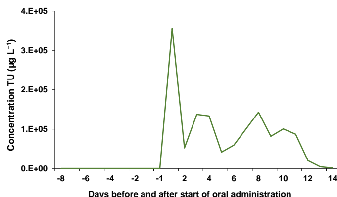
Figure 3.7. Excretion curve of Thiouracil.
