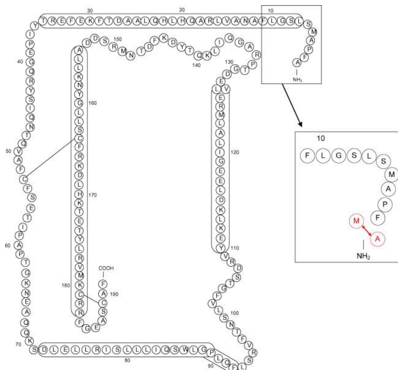
Figure 9.1. Schematic representation of the bovine growth hormone molecule with the N-terminal end in detail with the alanine (A) replaced by methionine (M) as in Monsanto recombinant rbST (Reproduced from [175]).
