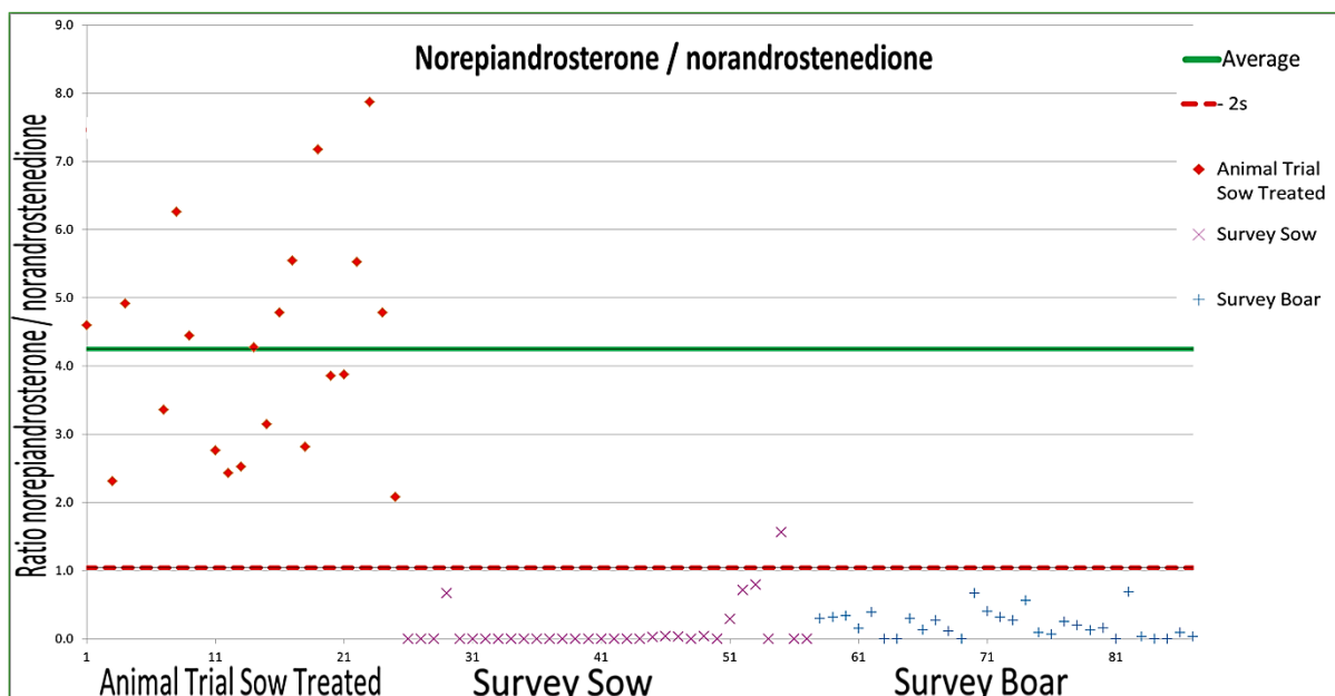
Figure 4.3. Profiling model to determine if 17\beta -NT is endogenous or exogenous based on the ratio of norepiandrosterone and norandrostenedione
