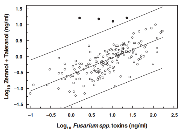
Figure 7.2. Graphical representation of the statistical model. The samples represented by a solid circle fell outside the 99% confidence interval and can be considered as suspect [139].
