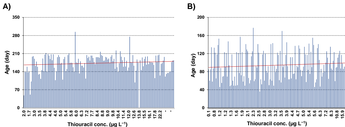
Figure 3.6. TU concentrations in (A) rosé meat animals and (B) white meat animals .
