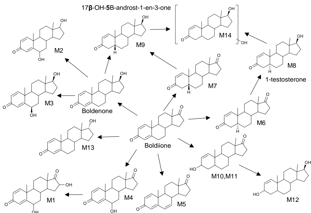
Figure 6.1. Overview of the metabolic pathway in humans of boldione [110].
