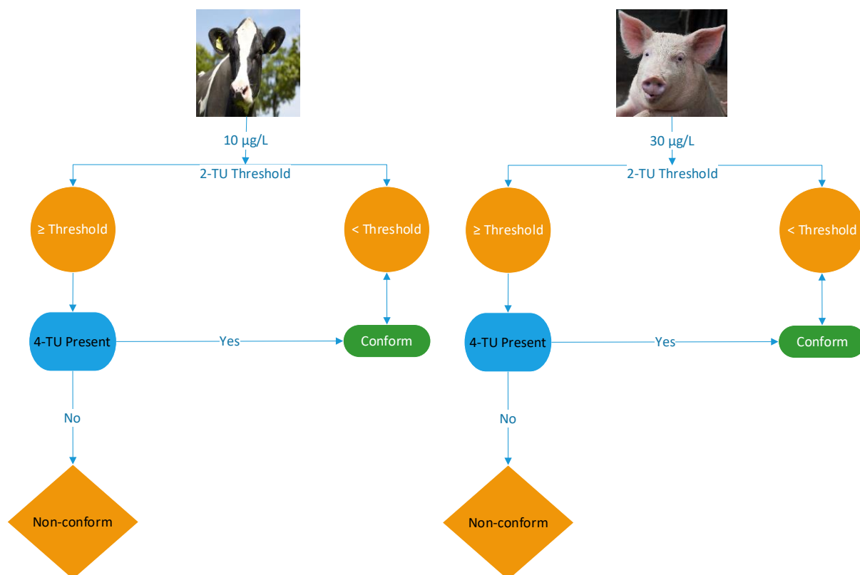
Figure 3.9. Flowchart Decision on Thiouracil finding in porcine and bovine animals.
