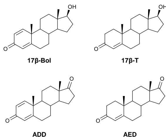
Figure 5.1. Structures of 17 \beta boldenone (17 \beta -Bol) and 17 \beta -testosterone (17 \beta -T) and of androsta-1,4-diene-3,17-dione (ADD) and androst-4-ene-3,17-dione (AED).
