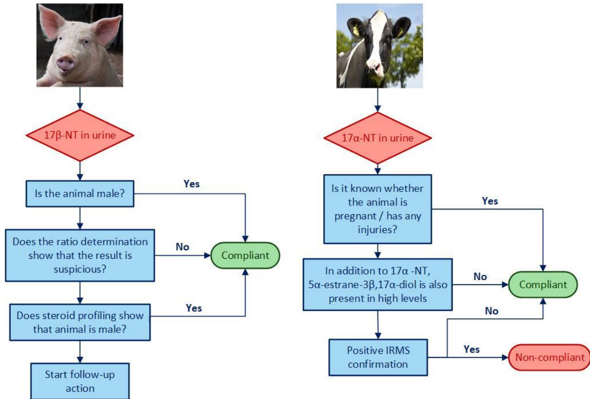
Figure 4.5. Flowchart Decision on nortestosterone finding in porcine and bovine animals.
