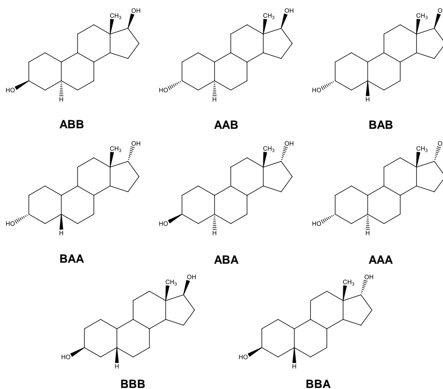
Figure 4.2. Chemical structures of the NT metabolites: estranediol isomers.
