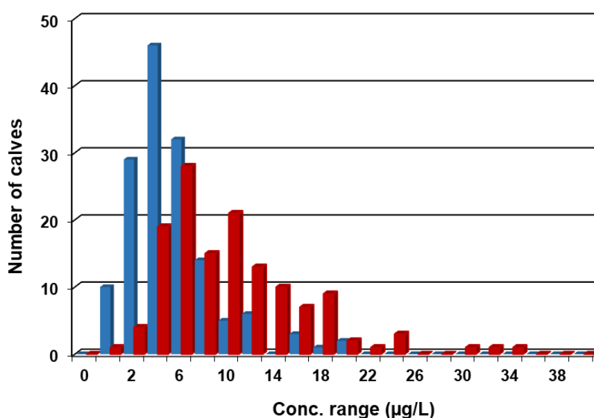
Figure 3.5. Distribution of TU concentration \mu\text{g L}^{-1} in urine of white meat (blue bars) and rosé meat (red bars) in calves in the Netherlands, monitoring May 2012.
