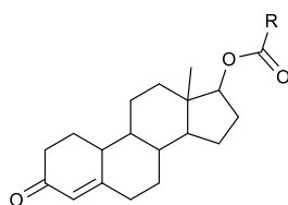
Figure 4.1. Structures of NT esters. NT-acetate: R=CH 3 , NT-benzoate: R=phenyl, NT-cypionate: C 2 H 4 -cyclopentyl, NT-hemisuccinate: CH 2 -succinyl, NT-decanoate: R=C 9 H 19 , NT-undecanoate: R=C 10 H 21 , NT-laureate: C 11 H 23 , NT-phenylpropionate: R=C 2 H 4 -phenyl, NT-propionate: R=C 2 H 5 .
