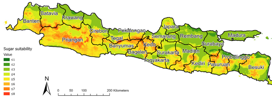
Fig. 7. Sugar Suitability across Java. Sources: Dippel et al. (2020); Jayasinghe and Yoshida (2010).
