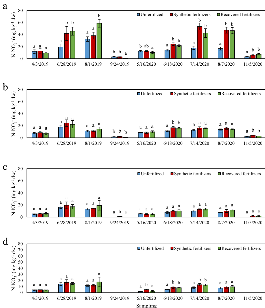
Fig. 1. Average concentration ( n = 3 ) of nitrate nitrogen ( \text{N-NO}_3^- ) in experimental soils in four layers with increasing depth, starting from the surface up to a depth of one meter (a: 0–25 cm from surface; b: 25–50 cm; c: 50–75 cm; d: 75–100 cm) during the 2019–2020 crop seasons. Error bars show Standard deviation. Letters are referred to One-way ANOVA ( p < 0.05 ; Tukey post-test), comparing the three values for each sampling.
