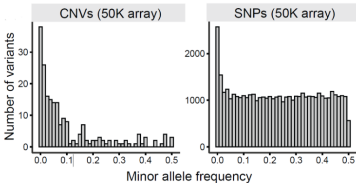
Figure 1. Minor allele frequency spectra of CNVs and SNPs obtained from the EuroGenomics array.
