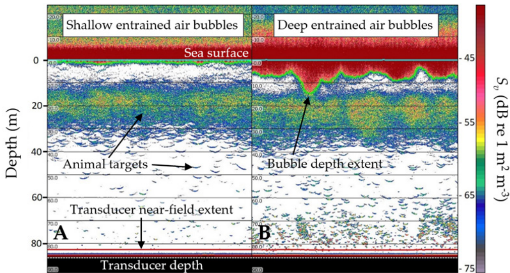
Figure 2.5. Calibrated measurements of S_v at 70 kHz from an upward-facing Simrad EK80 WBAT echosounder on the seabed at ~ 85 m depth in Holyhead Deep (Wales, UK). (A) A 5-min period of time on the 6 th of October 2019, when the depth of entrained air bubbles (green line) was at a minimum. (B) A 5-min period of time on the 8 th of October 2019, when the depth of entrained air bubbles (green line) extended to as much as ~ 15 m.
