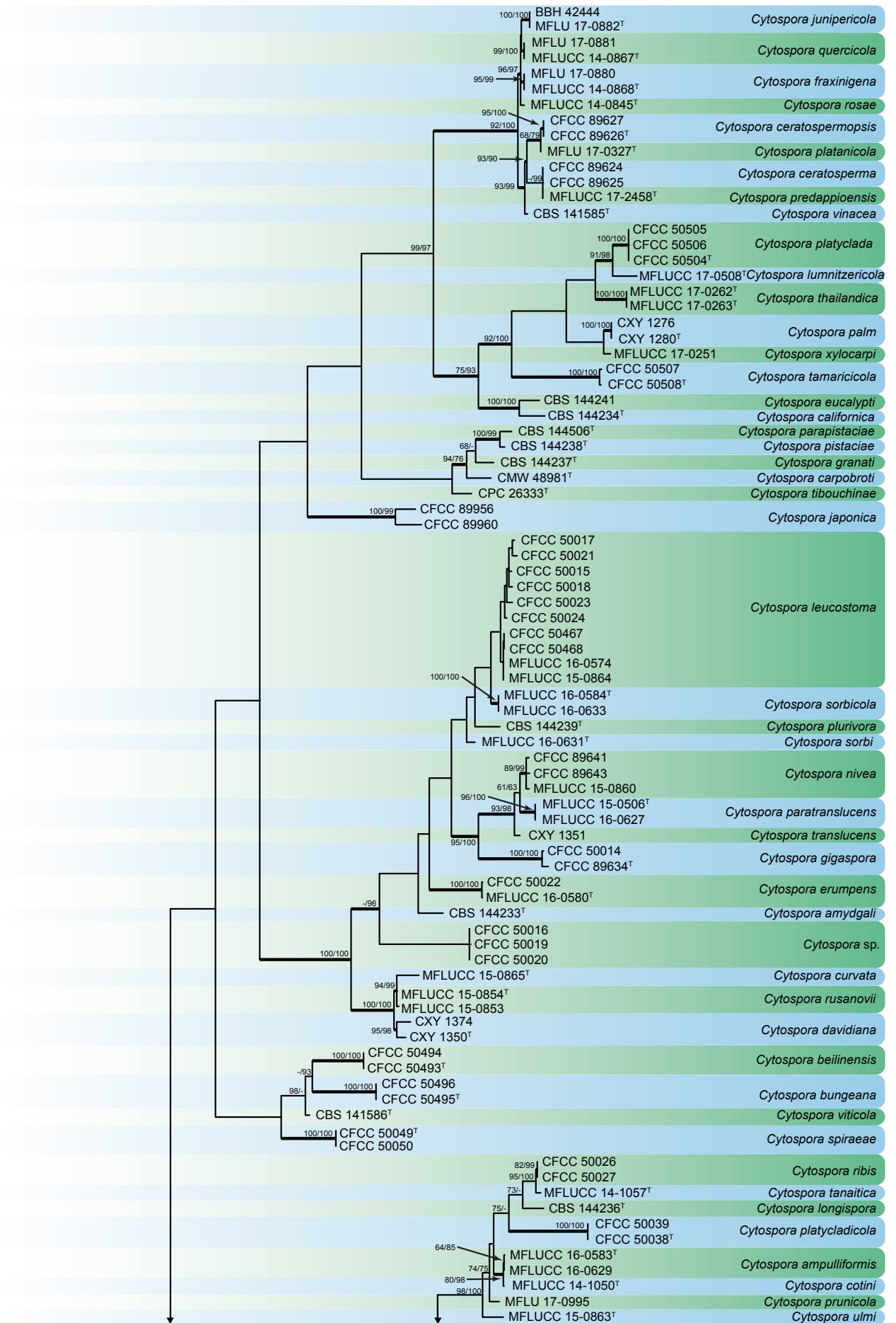
Fig. 19. Maximum parsimony phylogram constructed from ITS (662 bp), LSU (525 bp), act1 (357 bp), rpb2 (730 bp), tef1-α (796 bp) and tub2 (635 bp) sequences of all accepted species of Cytospora . Maximum parsimony (MP) and Maximum likelihood (ML) bootstrap support values (> 50 %) are shown at the nodes (MP/ML). Thickened branches represent Bayesian posterior probability scores (> 0.95). The phylogenetic tree was rooted to Diaporthe vaccinii CBS 160.32. GenBank accession numbers are indicated in Table 6. † indicates ex-type strains. TreeBASE: S26220.
