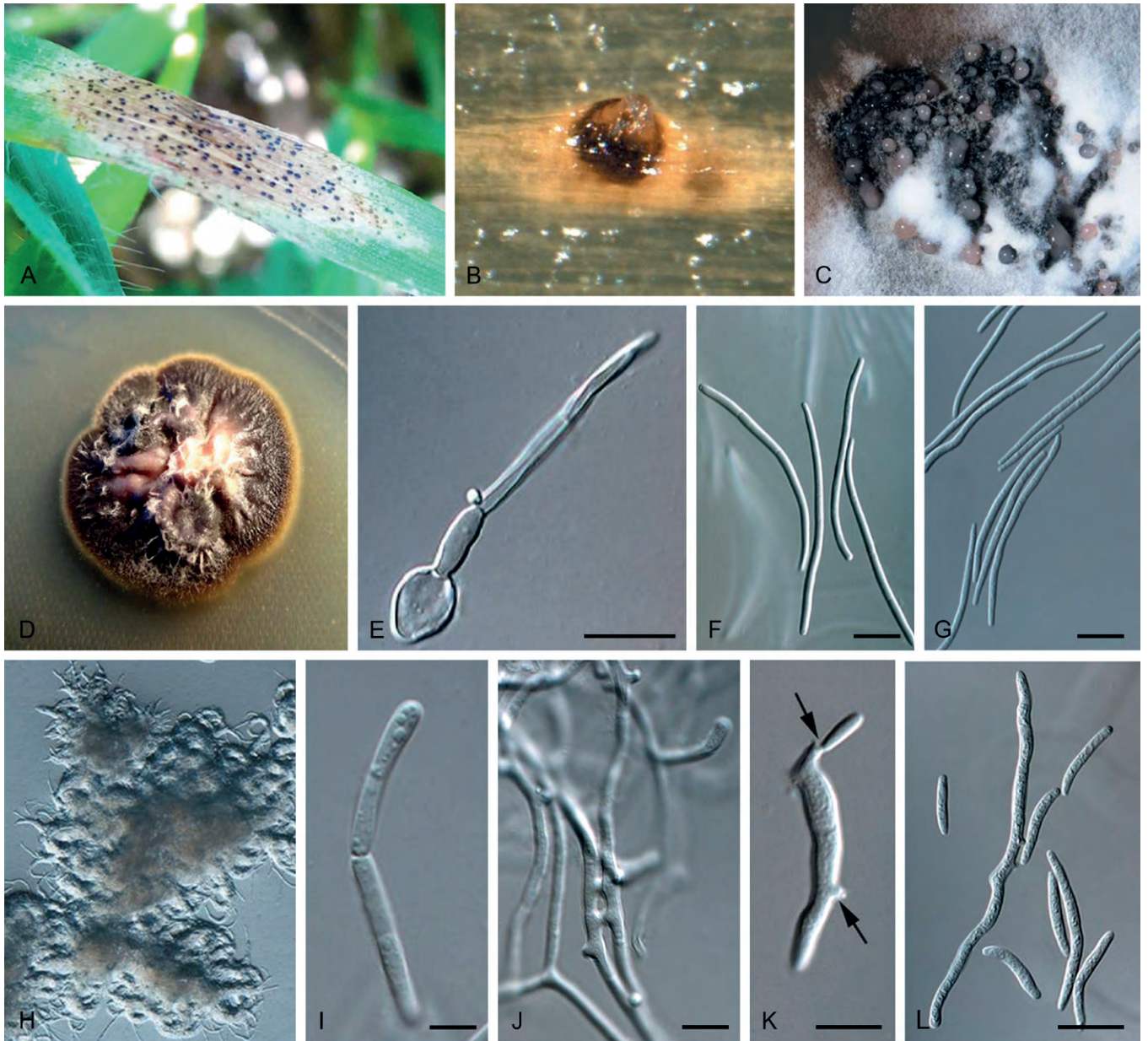
Fig. 71. Zymoseptoria spp. A, B. Disease symptoms. A. Zymoseptoria crescent (ex-type CBS 144410) on living leaves of Aegilops triuncialis . B. Zymoseptoria brevis (ex-type CBS 128853) forming a pycnidium on leaves of Hordeum vulgare . C, D. Colony sporulation on PDA. C. Zymoseptoria brevis (ex-type CBS 128853) colony with yeast-like growth on synthetic nutrient-poor agar. D. Zymoseptoria crescenta (ex-type CBS 144410) colony with yeast-like growth on synthetic nutrient-poor agar. E. Conidiogenous cell of Zymoseptoria passerinii (ex-epitype CBS 120382) formed inside pycnidium. F, G. Conidia (Type I). F. Zymoseptoria tritici (ex-epitype CBS 115943). G. Zymoseptoria halophila (ex-type CBS 128854). H. Zymoseptoria halophila (ex-type CBS 128854) colony with yeast-like growth on synthetic nutrient-poor agar. I, J. Conidia (Type II) of Zymoseptoria halophila (ex-type CBS 128854) formed as phragmospores in aerial hyphae. K, L. Conidia (Type III). K. Zymoseptoria brevis (ex-type CBS 128853) formed via microcyclic conidiation (arrows indicate Type III). L. Zymoseptoria tritici (ex-epitype CBS 115943). Scale bars = 10 µm. Pictures A, D taken from Crous et al. (2018c); B, C, E–L from Quaedvlieg et al. (2011).
