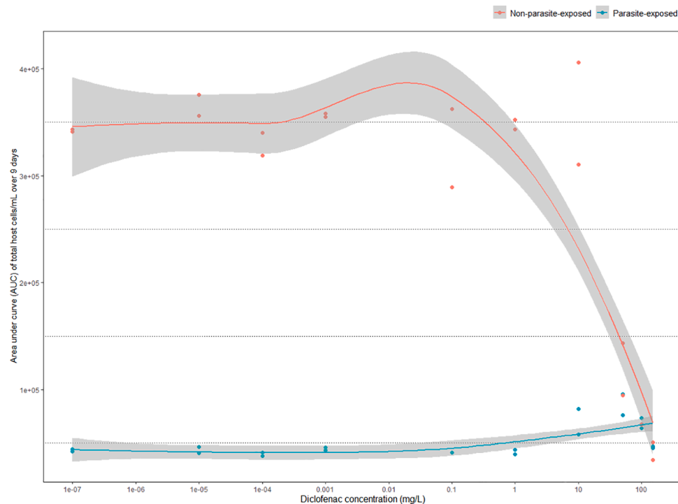
Fig. 3. Combined effect of Staurastromyces oculis parasite and diclofenac on Staurastrum host at 10 different diclofenac concentrations indicated by area under the curve of total host cells per mL over 9 days (AUC) in presence (blue dots) and absence (red dots) of Staurastromyces oculis parasite. Dashed lines indicate trends in AUC in presence (blue solid line) and absence (red solid line) of Staurastromyces oculis parasite with gray shaded areas indicating 95% confidence interval.
