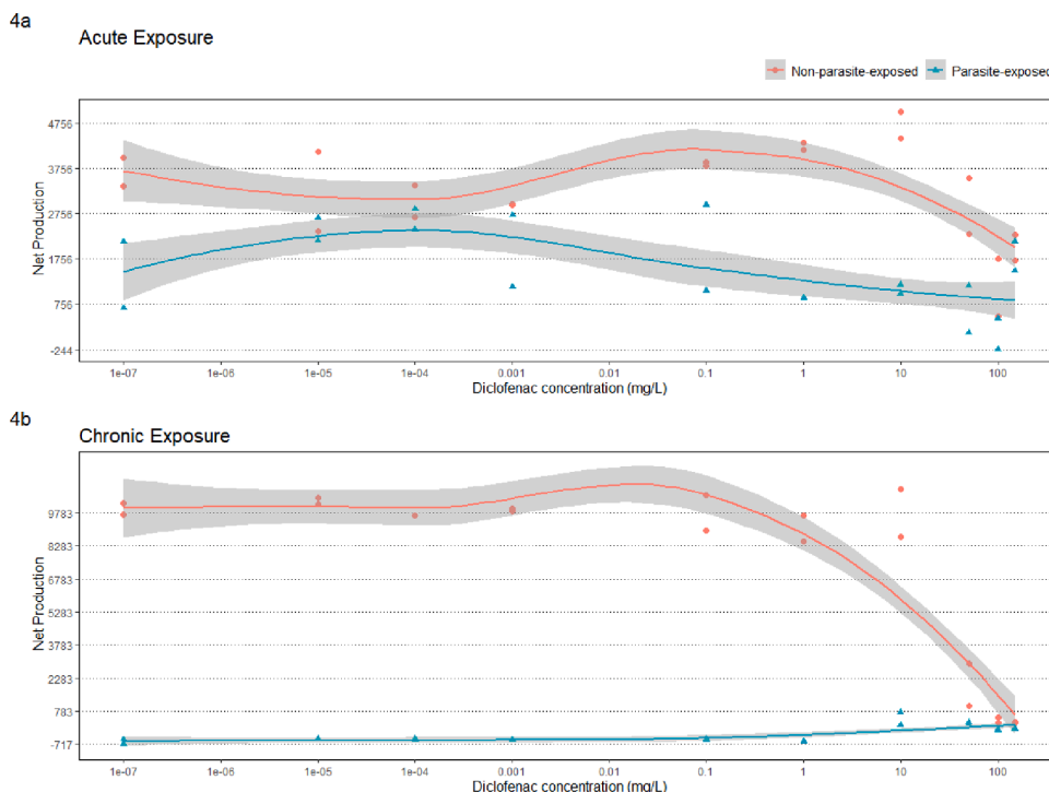
Fig. 4. Net production (host cells/mL over time) of 10 diclofenac concentrations (i.e. 0.1, 1, 10, 50, 100, 150 mg/L). (4a) Acute exposure: net production in non-parasite-exposed treatments (orange dots) and net production parasite-exposed treatments (blue triangles) over the first 48 h (4b) Chronic exposure: net production in non-parasite-exposed treatments (orange dots) and net production in parasite-exposed treatments (blue triangles) over 216 h (9 days). Dashed lines indicate trends in net production in presence (blue dashed line) and absence (red dashed line) of Staurastrumyces oculus parasite with gray shaded areas indicating 95% confidence interval.
