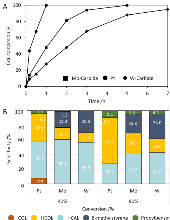
Fig. 2 (A) CAL conversion and (B) normalized product distribution at 40% and 90% conversion of CNF supported \text{MoC}_{1-x} , \text{W}_2\text{C} and Pt catalysts (50 ml toluene, 13.6 g per l CAL, T = 200^\circ\text{C} , 20 bar \text{H}_2 , 800 rpm).
