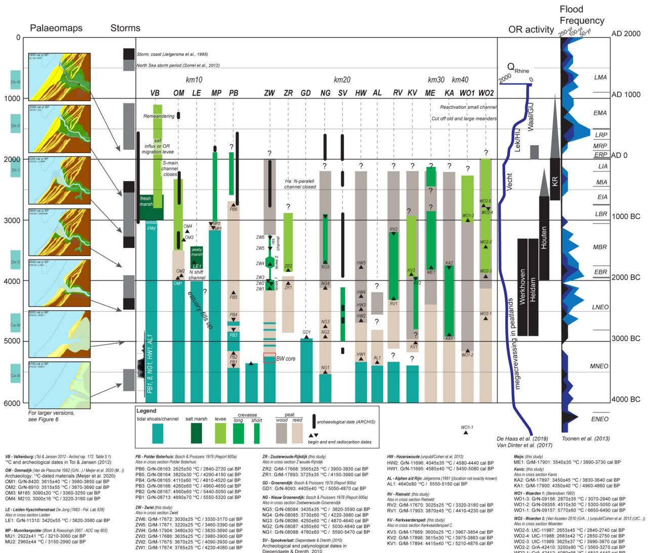
Fig. 9. Time–space diagram of overbank and floodbasin evolution along the Old Rhine (from ca 50 km upstream towards the coast) over the last 6000 years. Kilometre-positions and locations in Fig. 1. Calibrated radiocarbon dates (IntCal 2020) reported in 1 sig, rounded by 5. Most dates are also indicated in Table 3 and in cross-sections in Fig. 5. Dk/Ca = chronostratigraphical subdivision of The Netherlands (presumed transgression phases, in use until 2003) (Van der Valk, 1995). For Dutch archaeological periods see Table 4.
