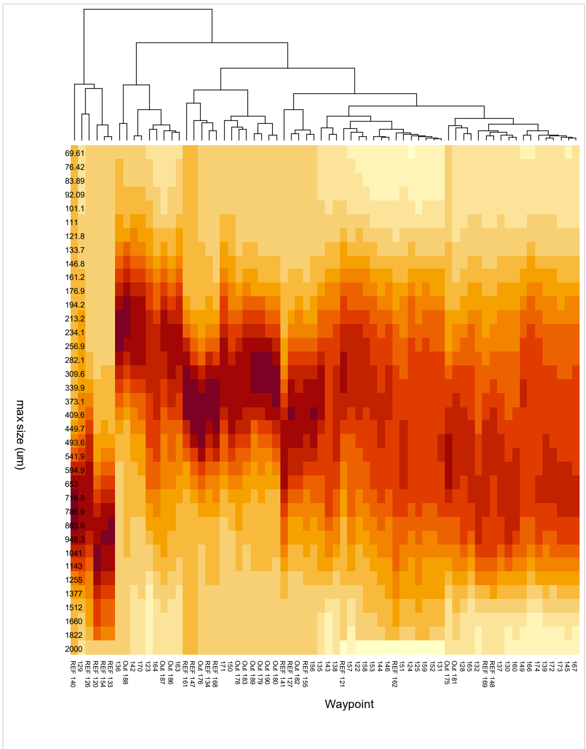
Figure 5. Heat map in which samples are grouped based on the grain size distribution of each sample. On the bottom, waypoint numbers are shown together with a label indicating whether the sample is considered a reference sample taken in front of Chogogo beach (REF), a sample from another beach (OUT), or taken at Chogogo beach (only a number). On the left side, the different size class border values are given, and the result of a grouping analysis is on top. The center image shows the percentage values within each size class, with darker colors indicating higher percentages.
