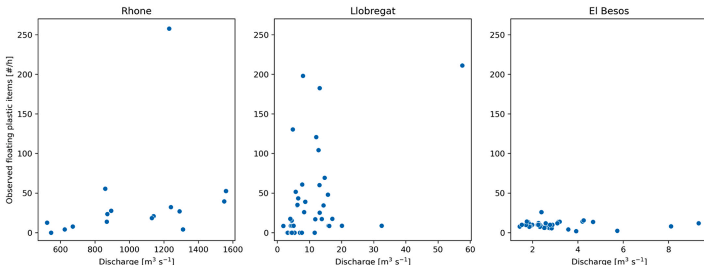
Fig. 1. Plastic flux observations and their corresponding river discharge for the Rhône, Besós and Llobregat rivers. Note the difference in scales on the x-axis.
