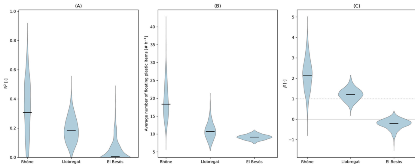
Fig. 4. (A) distribution of the R^2 values corresponding to the exponential regression (with environmental drivers) models linking non-linear discharge to the plastic flux, (B) distribution of averaged hourly predictions from the exponential regression models (from the whole year of predictions) and (C) distribution of the exponential parameter of the exponential regression model configurations for the different rivers. The black lines describe the modelling results on the original data.
