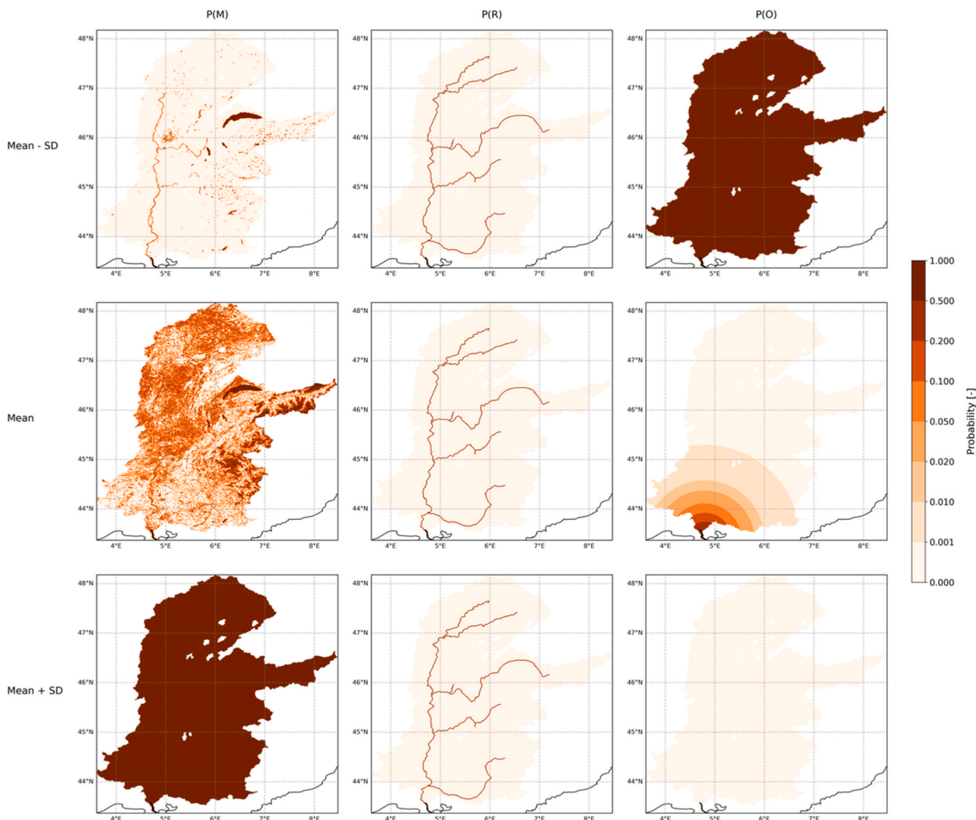
Fig. 5. Probability maps of mobilisation (P(M)), reaching the river network (P(R)) and reaching the river mouth (P(O)) for optimal parameters and parameters plus/minus one standard deviation. The plots represent the catchment of the Rhône river.
