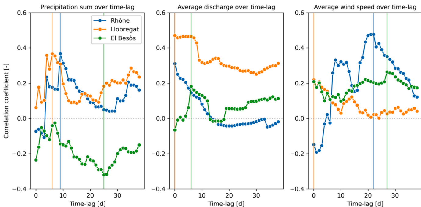
Fig. 3. Pearson correlation between floating macroplastic observations and hydrometeorological fluxes under different time-lags. The vertical lines depict the highest absolute correlation values per river-flux pair.
