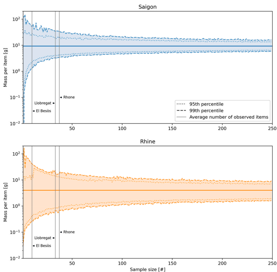
Fig. 2. Uncertainty in item-to-mass conversion. Estimated plastic mass as a function of sample size for the Saigon and Rhine rivers. The horizontal lines display the mean mass of all items in the two datasets (2123 and 452 items for Saigon and Rhine, respectively), which would be used as the item-mass conversion factor. The colored area above and below these lines display the area between the 1st and 99th percentile confidence interval from a bootstrap analysis. The uncertainty range (99th percentile divided by the 1st percentile) from mass conversion for the Rhône, Llobregat and Besós is 24, 34 and 151, respectively, when assuming a similar item-mass distribution to the Rhine. The vertical lines depict the average number of items found in the Rhône Llobregat and Besós rivers per monitoring session.
