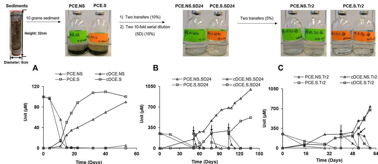
Figure 2. PCE dechlorination to cDCE in initial microcosms (A), serial dilutions (B) and further transfers (C) in the presence (S) and absence (NS) of sulfate. SD24: the fourth (i.e. 10^{-4} dilution) cultures in the second serial dilution in step 3 (Figure 1); Tr2: the second transfers in Step 4 (Figure 1). See also Figure 1 for a detailed scheme of the experimental set-up and history and relatedness of the different cultures. Vertical arrows indicate spikes of PCE. Data shown are average values, and error bars represent the standard deviation of the duplicates in Tr2. Error bars are not always visible due to small standard deviations.
