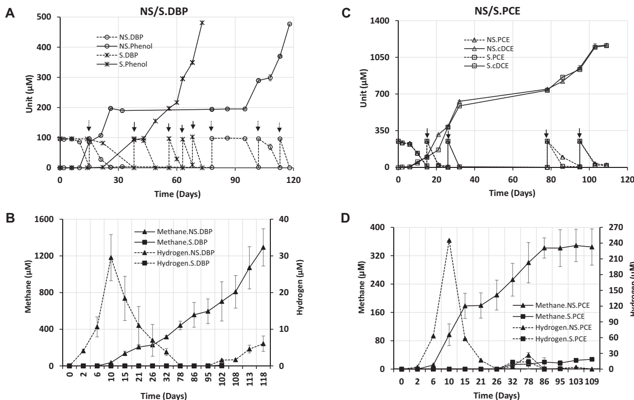
Figure 4. Reductive debromination of 2,6-DBP in addition to PCE dechlorination. In parallel cultures, 2,6-DBP and PCE are dehalogenated into phenol (A) and cDCE (C), respectively. Methane and hydrogen (B, D) are measured throughout the experiment in the presence or absence of sulfate. Values and error bars shown in the figure are averages and standard deviation of duplicate cultures. Arrows indicate the spikes of PCE (black) and 2,6-DBP (grey-dotted arrows for sulfate-free cultures, black for sulfate-amended cultures).
