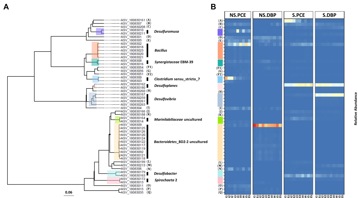
Figure 7. Phylogenetic analysis (A) and dynamics of microbial composition (B) at ASVs level. The cut-off relative abundance of ASVs is set at 0.1% in at least one single sample. ASVs belonging to the same genus are indicated by the same colour (top 10 genera) or letters. Alphabetic letters in Fig. 6A: A, Desulfobulbaceae ; B, Desulforhopalus ; C, Desulfobacterium ; D, Halodesulfobivrio ; E, Synergistaceae_uncultured ; F, Acholeplasma ; G, Mollicutes_EUB33-2_uncultured ; H, Desulfobivriales ; I, Desulfomicrobium ; J, Marinilabillaceae ; K, Bacteroidetes_vadinHA17 ; L, Lentimicrobiaceae ; M, VC2.1_Bac22_uncultured ; N, VC2.1_Bac22 ; O, Bacteria_LCP-89 ; P, Methanogenium ; Q, Methanomicrobiaceae ;
