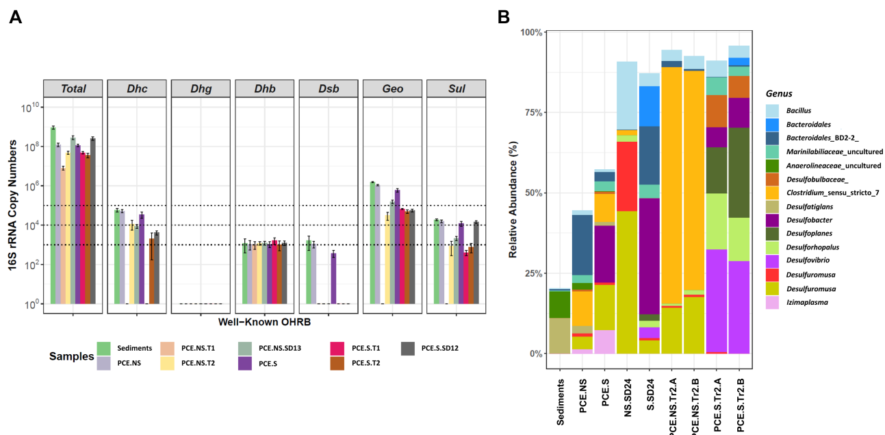
Figure 3. Microbial community analysis of PCE-dechlorinating cultures by qPCR (A) and 16S rRNA gene amplicon sequence data at genus level (B). 16S rRNA gene copy numbers per millilitre of the cultures except for the marine sediments (Sediments) that are defined per gram of wet sediment. Total: total bacterial 16S rRNA gene copy numbers; Dhc: Dehalococcoides; Dhg: Dehalogenimonas; Dhb: Dehalobacter; Dsb: Desulfobacterium; Geo: Geobacter; Sul: Sulfurospirillum. Values and error bars represent the averages and standard deviations of the triplicate qPCRs, respectively. Values below the detection limit are shown as one copy per ml. The added horizontal dotted lines represent 10^3 , 10^4 , and 10^5 copy numbers, respectively. Only taxa that have a relative abundance > 5% in at least one of the samples are shown. Duplicate enrichments are indicated by suffixes 'A' and 'B'. T1 and T2: the first and second transfers in step 2 (Figure 1); SD12 and SD13: the second ( 10^{-2} ) and third ( 10^{-3} ) dilution cultures in the presence and absence of sulfate, respectively, in the first serial dilution in step 3 (Figure 1). See also Figure S2.
