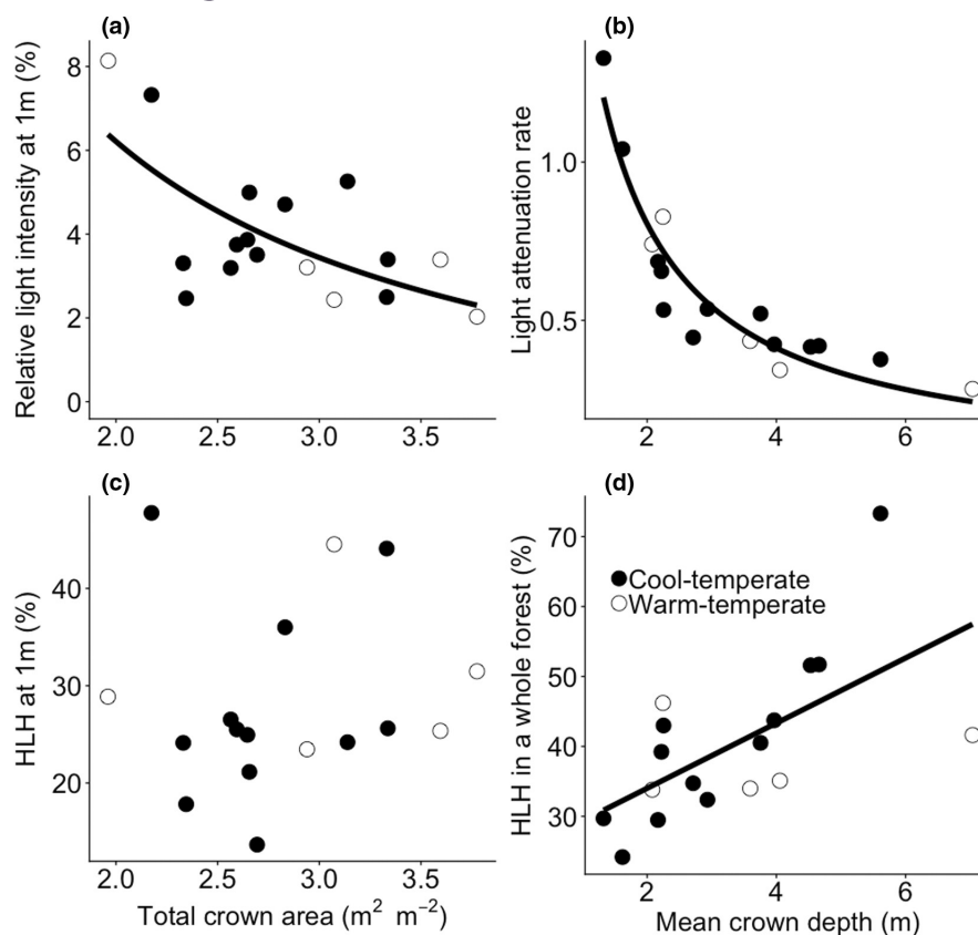
FIGURE 4 Forest light attributes in relation to forest structural attributes across forest stands of different ages in cool- and warm-temperate climates. (a) The relative light intensity (RLI) at 1 m above the ground plotted against the total crown area per unit of ground area; (b) the light attenuation rate (i.e., the rate of light extinction with height) plotted against the mean crown depth; (c) horizontal light heterogeneity (HLH) at 1 m above the ground (coefficient of variation of RLI at 1 m above the ground across 16 subplots) plotted against the total crown area per unit of ground area; and (d) the HLH of a whole forest (the mean value of the coefficient of variation of RLI across all height classes among 16 subplots in each plot) plotted against the mean crown depth. In (a,b,d), a single regression line was drawn for pooled data because there was no difference between the cool- and warm-temperate forests. The detailed model results can be found in Appendix S8 . Regression lines are (a) y = 16.62/x - 2.10 ; (b) y = 1.57/x + 0.020 ; (d) y = 4.66x + 24.69
