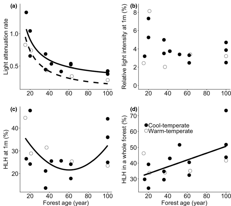
FIGURE 3 Successional trajectories of the forest light attributes in cool- and warm-temperate forests: (a) light attenuation rate (i.e., the rate of light extinction by height); (b) relative light intensity at 1 m above the ground; (c) horizontal light heterogeneity (HLH) at 1 m above the ground (the coefficient of variation of the relative light intensity at 1 m above the ground across 16 subplots); and (d) the HLH of a whole forest (the mean value of the coefficient of variation of relative light intensity across all height classes among 16 subplots in each plot) plotted against the different stand ages. In (a), continuous lines represent the regression lines of the cool-temperate forest, and hatched lines represent the regression lines of the warm-temperate forest. In (c, d), a single regression line was drawn for pooled data because there was no difference between the cool- and warm-temperate forests. The detailed model results can be found in Appendix S6 . Regression lines are (a) cool: y = 12.78/x + 0.27 , warm: y = 12.67/x + 0.098 ; (c) y = 0.0068x^2 - 0.83x + 46.47 ; (d) y = 0.22x + 29.03
