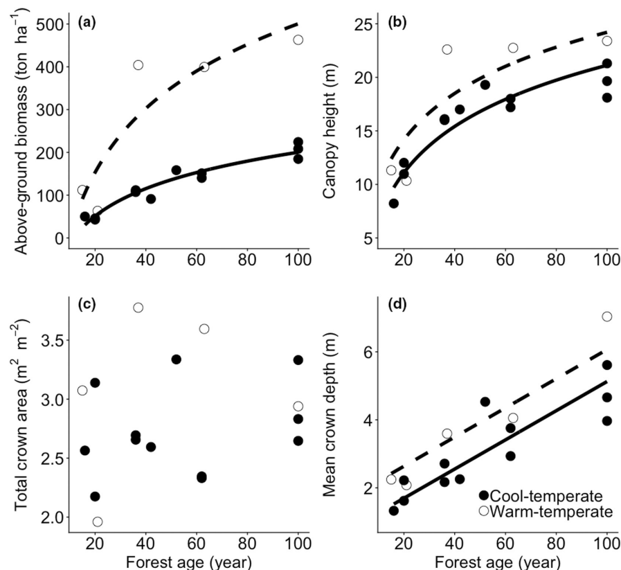
FIGURE 1 Successional trajectories of forest structural attributes in cool- and warm-temperate forests: (a) total above-ground biomass; (b) canopy height of the forest; (c) total crown area per unit of ground area; and (d) mean crown depth plotted against forest age. Continuous lines represent the regression lines for the cool-temperate forests, and hatched lines represent the regression lines for the warm-temperate forests. The detailed model results can be found in Appendix S3 . Regression lines are (a) cool: y = 213.44 \log_{10}(x) - 226.65 , warm: y = 497.04 \log_{10}(x) - 493.59 ; (b) cool: y = 14.35 \log_{10}(x) - 7.57 , warm: y = 14.35 \log_{10}(x) - 4.49 ; (d) cool: y = 0.043x + 0.84 , warm: y = 0.043x + 1.78
