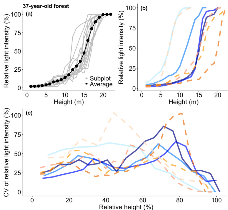
FIGURE 2 Forest light profiles at four secondary successional stages (early, mid-early, middle, and late) in cool- and warm-temperate forests. (a) An example of vertical light profiles in a plot (37-year-old forest stand in the warm-temperate forest); (b) average vertical light profiles per plot ( n = 16 per plot) in stands of different age; and (c) the coefficient of variation (cv) of the relative light intensity among 16 subplots for a given height in relation to relative height (%) — that is, with the highest tree per plot normalized to 100%. In (b) and (c), only one representative plot per successional stage in each forest type is shown; blue solid lines represent the cool-temperate forest and orange dashed lines the warm-temperate forest. The lighter color indicates the plots in early successional stages whereas the darker color indicates the plots in late successional stages
