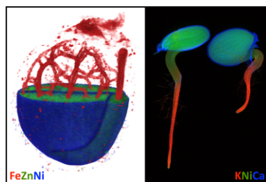
Tomographic reconstruction and 2D elemental mapping of Noccaea caerulescens seeds.
