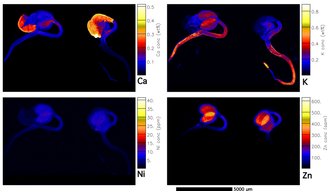
Fig. 6 Elemental X-ray fluorescence microscopy (XFM) maps of living Nocca caerulea seedlings (Ganges accession, non-ultramafic, calamine). The scan size is 21.8 × 31 mm (2366 × 1562 pixels). The elemental image was acquired in 5 μm step size with 2.5 ms dwell per pixel, 15.8 keV, incident beam, showing K, Ca, Ni, and Zn maps.
