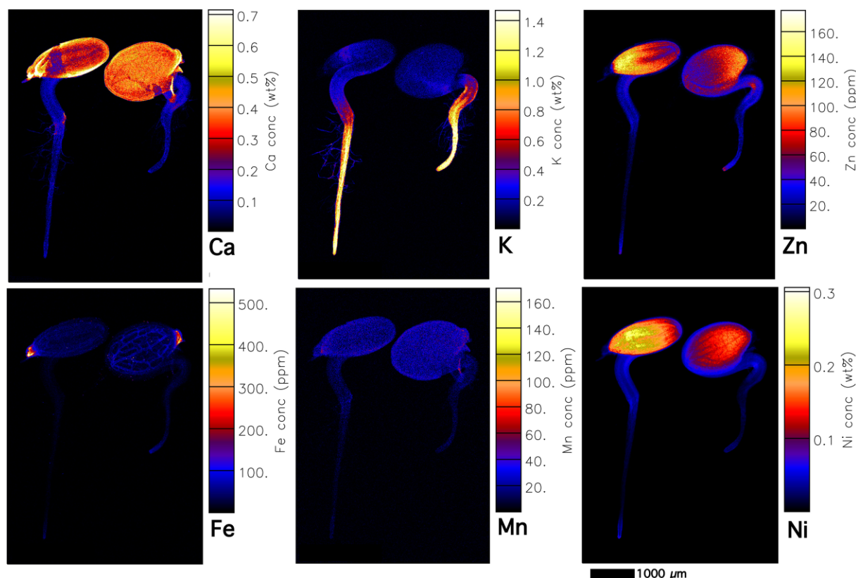
Fig. 4 Elemental X-ray fluorescence microscopy (XFM) maps of living Nocca caerulescens seedlings (Vosges accession, ultramafic). The scan size is 44 \times 9.8 mm ( 885 \times 1240 pixels). The elemental image was acquired in 5 \mu\text{m} step size with 2.5 ms dwell per pixel, 15.8 keV, incident beam, showing K, Ca, Fe, Mn, Ni, and Zn maps.
