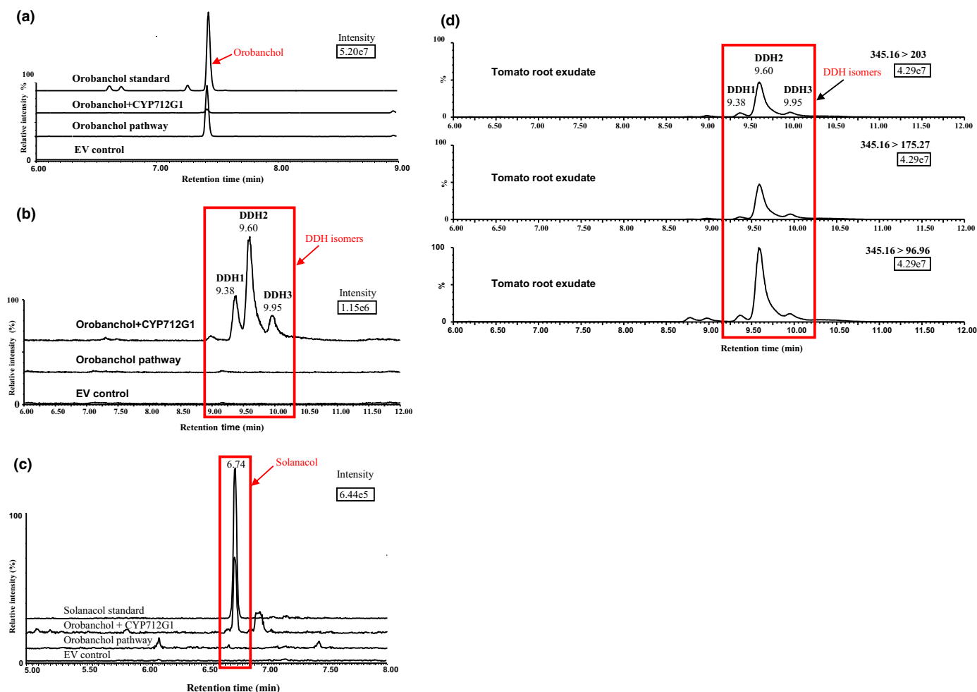
Fig. 3 Biochemical characterisation of CYP712G1 using transient expression in Nicotiana benthamiana . (a) The reduction of orobanchol (transition [M+H]^+ m/z orobanchol 347.2 > 97) in the transient expression assay. (b) The multiple reaction monitoring (MRM) chromatogram of dihydro-orobanchol (DDH) isomers (transition [M+H]^+ m/z 345.16 > 96.96) on enantio-selective column in transient expression assay. (c) The production of solanacol (transition [M+H]^+ m/z 343.16 > 96.97) in the transient expression assay. (d) The MRM chromatogram of DDH isomers (transition [M+H]^+ m/z 345.16 > 96.96, 345.16 > 175.27 and 345.16 > 203) on enantio-selective column in tomato root exudate under aeroponic system. EV, empty vector; orobanchol pathway, SID27 + SICCD7 + SICCD8 + Os900 + Os1400 ; orobanchol + CYP712G1 , co-expression of CYP712G1 with the orobanchol pathway.
