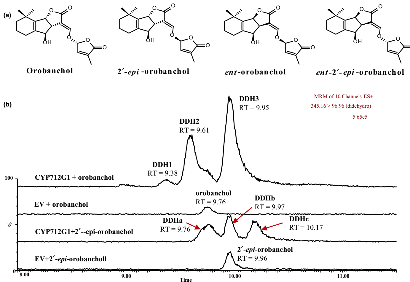
Fig. 5 Multiple reaction monitoring-liquid chromatography tandem mass spectrometry (MRM-LC/MS/MS) identification of didehydro-orobanchol (DDH) isomers and orobanchol stereoisomers of yeast microsomes in vitro assay on enantio-selective column. (a) Structures of orobanchol stereoisomers. (b) Representative chromatogram of the production of DDH isomers (transition [M+H]^+ m/z DDH_345.16 > 96.96) in the enzyme assay mixture with yeast microsomes expressing CYP712G1 (empty vector (EV) as control) and two orobanchol isomers after incubation of 3 h as analysed using MRM-LC-MS ( n = 3 ) on an enantio-selective column.
