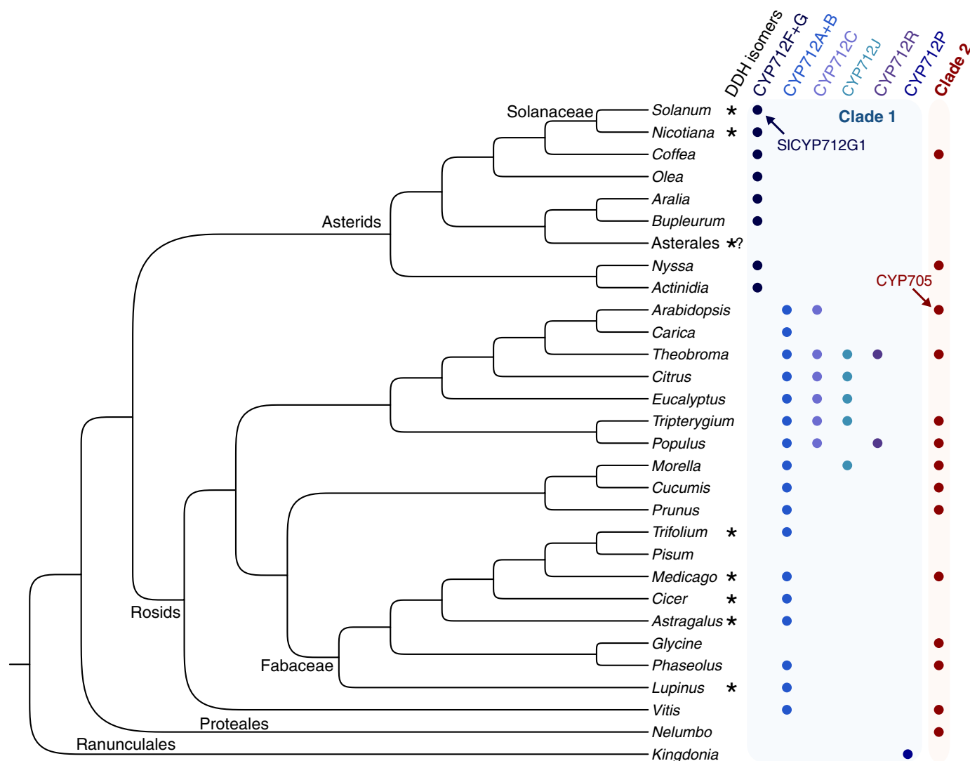
Fig. 7 Distribution of the CYP712 gene subfamilies across the Eudicot phylogenetic tree. Asterisks indicate described presence of didihydro-orobanchol (DDH) isomers. The black and red arrows indicate tomato ( Solanum lycopersicum ) CYP712G1 and Arabidopsis CYP705 subfamilies, respectively.
