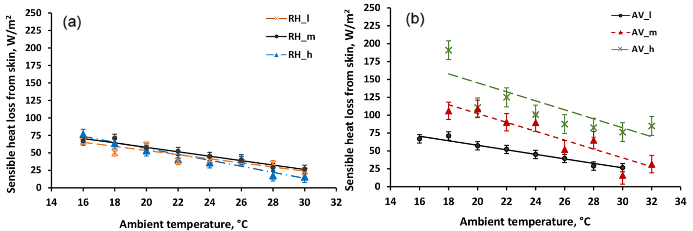
Figure A1. Sensible heat loss from the skin surface under short exposure in relation to ambient temperature (a) at the same air velocity levels (0.1 m/s) with low ( RH_l ; 30%), medium ( RH_m ; 45%), and high ( RH_h ; 60%) relative humidity, and (b) at the same relative humidity level (45%) with low ( AV_l ; 0.1 m/s), medium ( AV_m ; 1.0 m/s), and high ( AV_h ; 1.5 m/s) air velocity levels. Error bars represent SEM.
