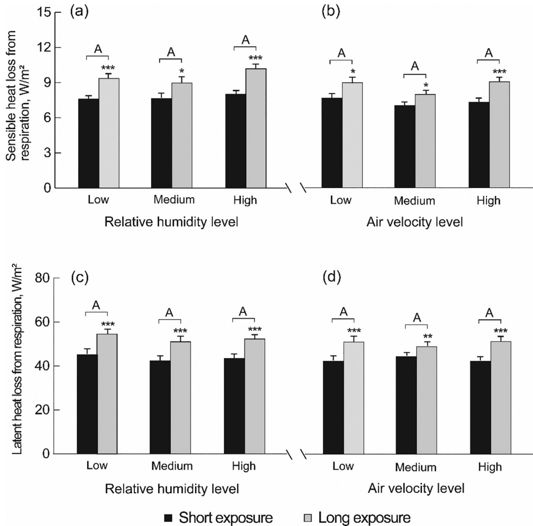
Figure 8. Mean sensible heat loss from respiration (a and b, \text{W/m}^2 ) and mean latent heat loss from respiration (c and d, \text{W/m}^2 ) within the ambient temperature range of 18 to 30^\circ\text{C} at short and long exposure times with different relative humidity (RH) levels (low, medium, and high) and air velocity (AV) levels (low, medium, and high). The different letters in the same variable indicate a significant difference (Tukey-Kramer, P < 0.05 ) between treatments. Asterisks indicate a significant difference between 2 exposure times ( *P < 0.10 , **P < 0.05 , ***P < 0.01 ). Error bars represent SEM. The RH effects were studied at low AV, and AV effects were studied at medium RH; the medium RH levels (a, c) are the same treatment as the low AV levels (b, d).
