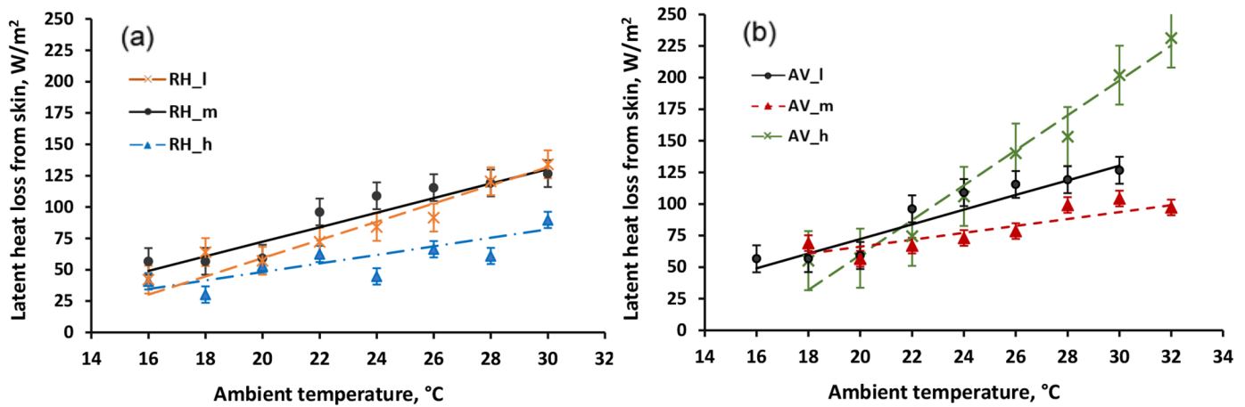
Figure A2. Latent heat loss from the skin surface under short exposure in relation to ambient temperature (a) at the same air velocity levels (0.1 m/s) with low ( RH_l ; 30%), medium ( RH_m ; 45%), and high ( RH_h ; 60%) relative humidity, and (b) at the same relative humidity level (45%) with low ( AV_l ; 0.1 m/s), medium ( AV_m ; 1.0 m/s), and high ( AV_h ; 1.5 m/s) air velocity levels. Error bars represent SEM.
