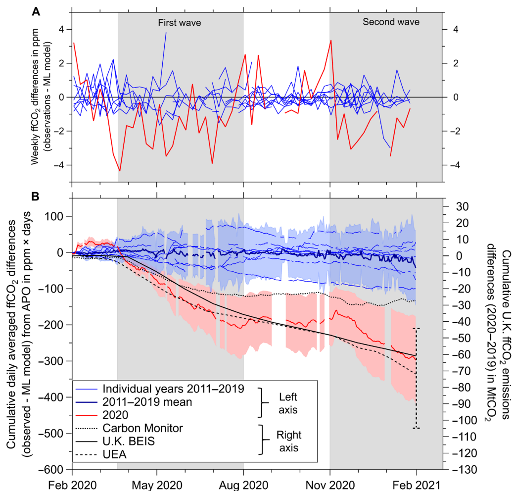
Fig. 3. Reduction in WAO ffCO 2 associated with COVID-19 lockdowns. (A) Differences in ffCO 2 [as ffCO 2 determined from APO minus modeled ffCO 2 determined from a random forest machine learning (ML) algorithm], shown as weekly differences. The first and second U.K. COVID-19 waves are indicated by the gray background shading. Differences for the individual years 2011–2019 are shown in blue. The period February 2020 to January 2021 is shown in red. All units are parts per million; x-axis major tick marks denote the first day of the month. Uncertainties are omitted from this panel for clarity. (B) Same as (A), but shown as cumulative daily-averaged ffCO 2 in units of parts per million × days. The thick blue line indicates the 2011–2019 mean. Uncertainties are as follows: The blue shading is the \pm 2\sigma (95%) SD of the 2011–2019 mean, shown by the thick blue line, and represents the uncertainty of the training model (i.e., if the model performance was perfect, then the blue lines would all be zero), which, in part, arises from the long-term decreasing trend in U.K. emissions over the period 2011–2019; ffCO 2 uncertainty for February 2020 onward is shown by the pale red shading and arises from the poorer performance of the predictive model relative to the training model (see the “Analysis of uncertainties” section for details). For comparison with our ffCO 2 [APO] detected COVID-19 signal, we also show 2020–2019 differences from three bottom-up U.K. emissions estimates (black lines) on the right-hand axis in units of MtCO 2 (see Materials and Methods). Only the UEA value (black dashed line) includes an estimate of uncertainty, shown by the vertical error bar.
