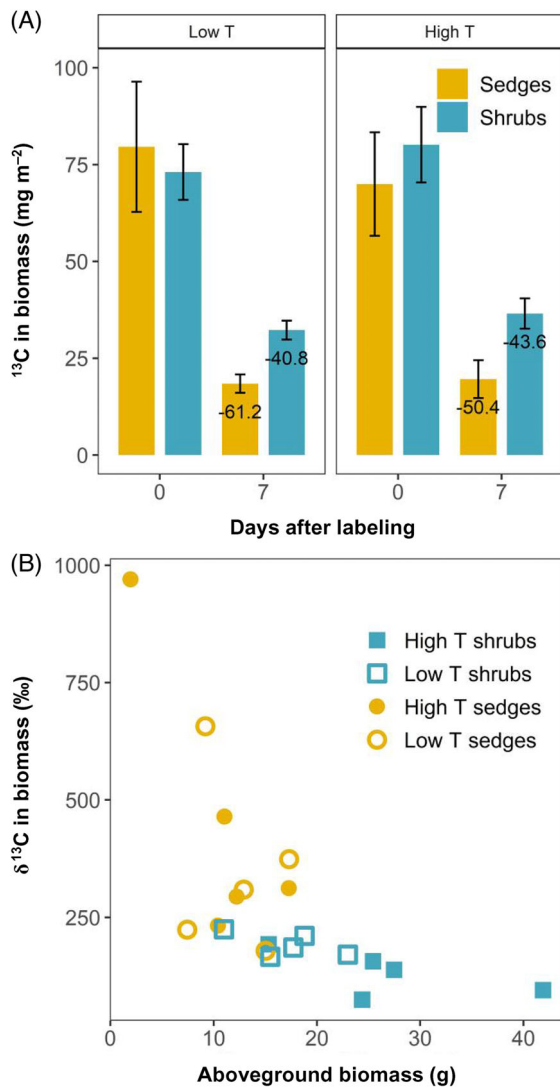
FIGURE 1 (A) Retained amounts of ^{13}\text{C} in aboveground biomass of shrubs ( C. vulgaris ) and sedges ( E. vaginatum ) at two peatland sites (high and low temperature sites, high temperature (T) and low T, respectively) directly (day 0) and 7 days after labelling. Numbers in the figure represents the relative loss of ^{13}\text{C} in the aboveground biomass from 0 to 7 days after labelling. (B) Inverse relationship between the enrichment in \delta^{13}\text{C} of shoot biomass of shrubs and sedges directly after labelling (day 0) and shoot biomass per plot at two peatland sites differing in temperature (high and low temperature sites, high T and low T, respectively)
