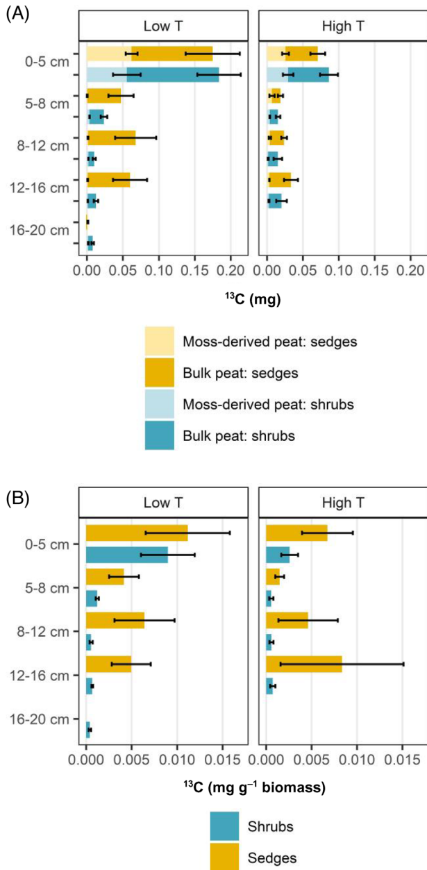
FIGURE 4 (A) Belowground allocated ^{13}\text{C} in peat cores sampled on the second day after labelling at two peatland sites (high and low temperature sites, high temperature (T) and low T, respectively) under shrubs and sedges. Stacked bars represent means with standard error (SE) per increment of moss-derived peat subsample and bulk peat subsample under the respective vascular plant. Moss-derived peat represents pure residues of moss (without any visible vascular plant constituents), whereas bulk peat represents both residues of vascular plant tissues and moss-derived peat. (B) Belowground allocated ^{13}\text{C} per gram aboveground biomass in peat cores sampled on the second day after labelling at two peatland sites (high and low temperature sites, high T and low T, respectively) under shrubs and sedges. Bars represent means of ^{13}\text{C} in the bulk peat subsamples divided by the amount of aboveground biomass
