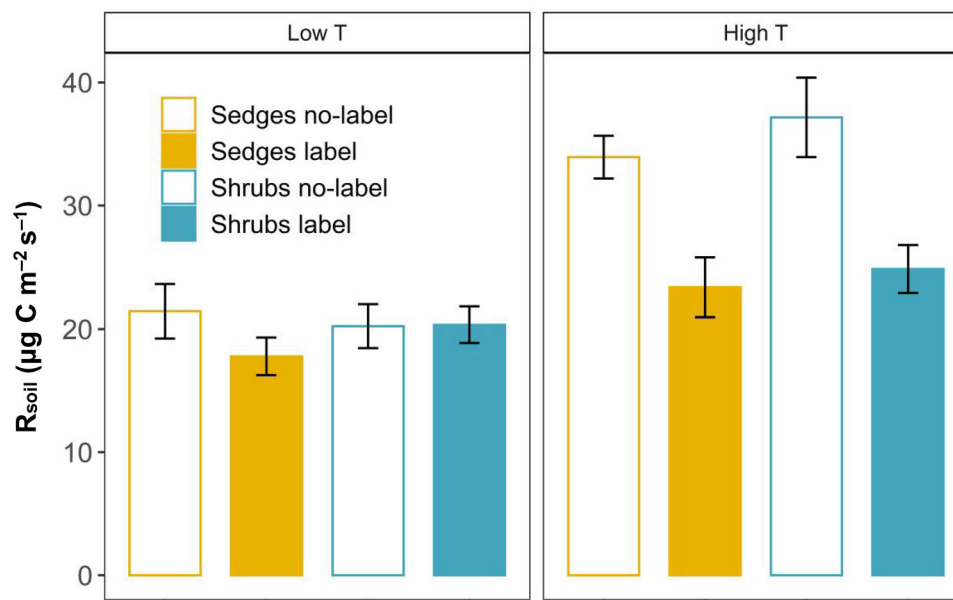
FIGURE 2 Mean soil respiration rates over 7 days after labelling for the label and no-label plots of shrubs ( C. vulgaris ) and sedges ( E. vaginatum ) at two peatland sites (high and low temperature sites, high temperature (T) and low T, respectively)
