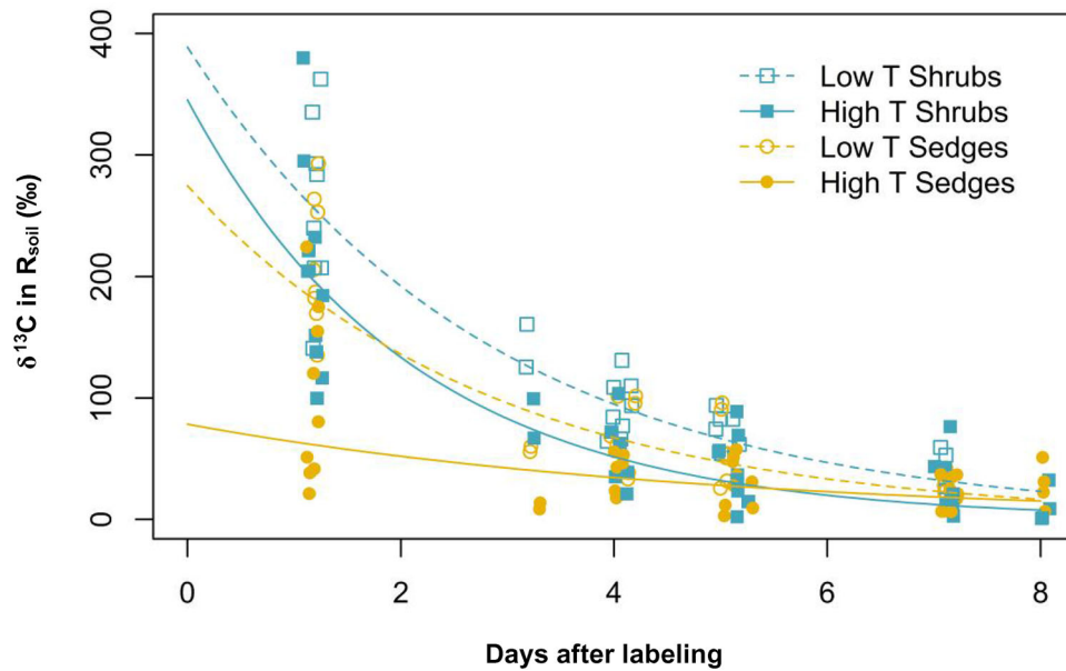
FIGURE 3 Decrease of \delta^{13}\text{C} in soil respiration described by exponential decay function for shrubs ( C. vulgaris ) and sedges ( E. vaginatum ) at two peatland sites differing in temperature (high and low temperature sites, high T and low T, respectively). Decay functions were fitted to data past 24 h after labelling
