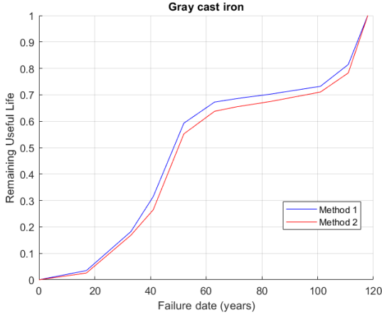
Fig. 2. RUL based on Weibull and CoxMLP.
