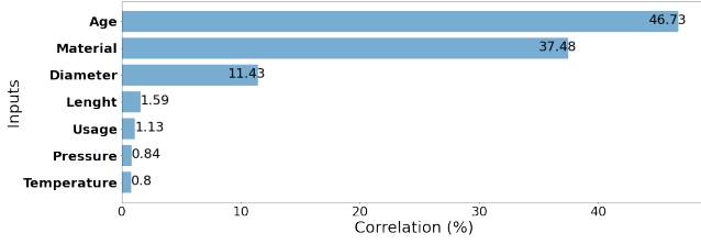
Fig. 1. Importance of different factors for failure rate.
