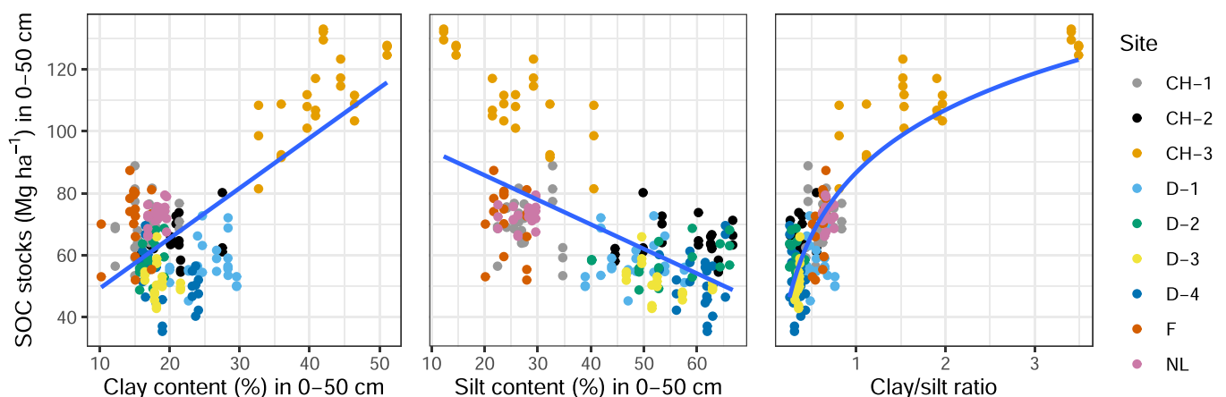
Fig. 4. Regressions of SOC stocks (Mg ha -1 ) in 0–50 cm calculated by the fixed depth (FD) approach with clay and silt content (%) and the clay-silt ratio across nine field trials.
