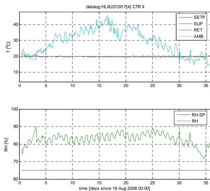
Figure 6 data registered by reefer unit in HLXU3729174 (125 m 3 /h).
