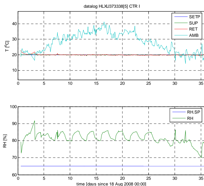
Figure 5 data registered by reefer unit in HLXU3733385 (100 m 3 /h).
