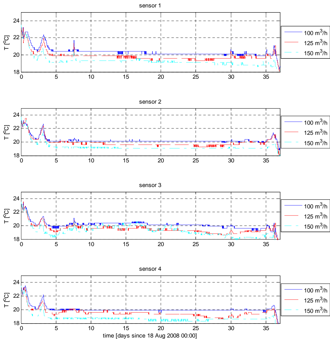
Figure 2 temperatures registered at the 4 locations indicated in Figure 1 throughout voyage.
