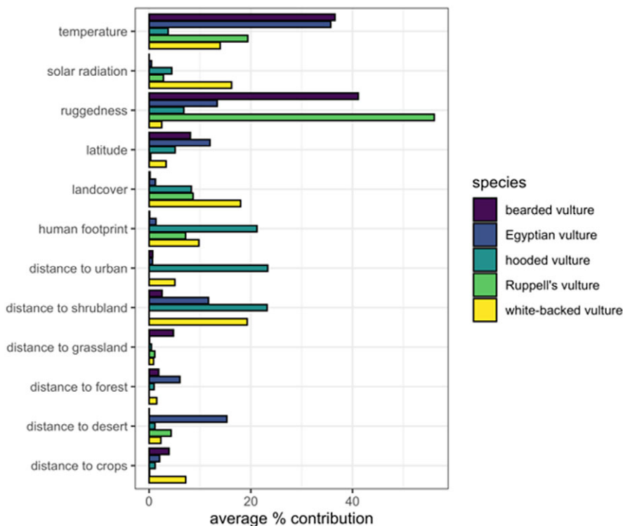
Figure 2. Average percent contribution of each predictor variable to the final ensemble distribution model for each species.
