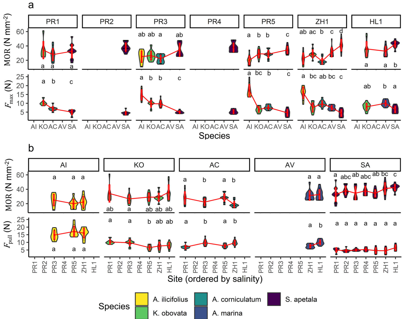
Fig 5. MOR (N mm -2 ) and leaf strength F_{pull} (N) across (a) species per site and (b) sites per species, with sites ordered toward increasing salinity (salinity based on Fig. 1). Letters indicate significance following Dunn's test with \alpha = 0.05 (for A. marina a t-test was used), letters should be read per individual plot only (considering 24 plots in total).
