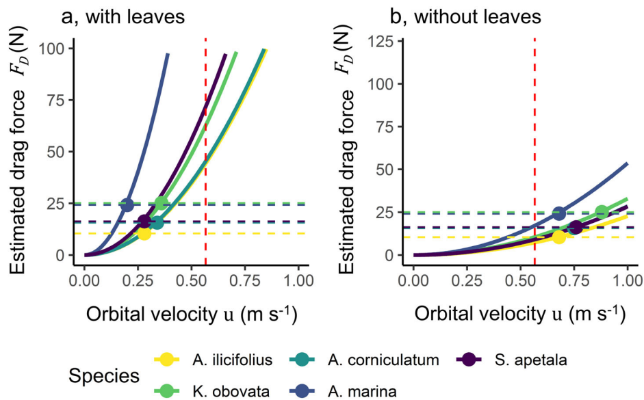
Fig 7. Conceptual model with estimations of drag force F_D experienced for idealized branches of 1 cm in diameter \phi , (a) with and (b) without leaves. Dashed lines indicated maximum force F_{\max} a branch can withstand. Red dotted lines indicate estimated peak orbital velocity during a typhoon (based on Hato, August 2017). See Supporting information, Appendix S1 for calculation.
