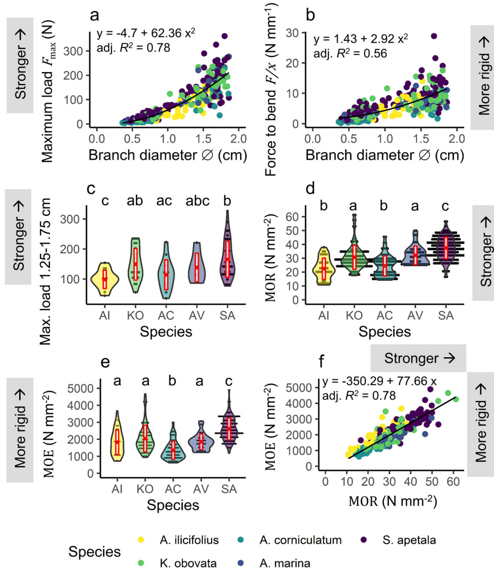
Fig 2. Branch mechanical properties of five mangrove species with (a) maximum load before breaking ( F_{\max} ; N) per diameter \phi (cm), (b) force needed to bend the branch ( F/x ; \text{N mm}^{-1} ) per diameter \phi (cm), (c) the maximum load F_{\max} (N) for branches ranging from 1.25 to 1.75 cm, (d) average MOR ( \text{N mm}^{-2} ), (e) average MOE ( \text{N mm}^{-2} ), and (f) MOE vs. MOR. Red crossbars indicate mean and standard deviation. Letters indicate significance following Dunn's test with \alpha = 0.05 .
