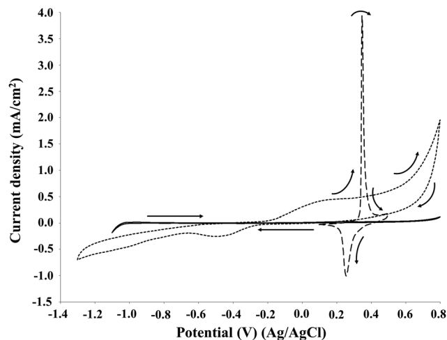
Fig. 3 Cyclic voltammetry of 2 \text{ g L}^{-1} P1000 lignin in 1 \text{ M NaOH} (pH 14). Voltammograms recorded at 10 \text{ mV s}^{-1} at room temperature. Solid line: on platinum electrode; dashed line: on NiOOH electrode; dotted line: on graphite electrode.
