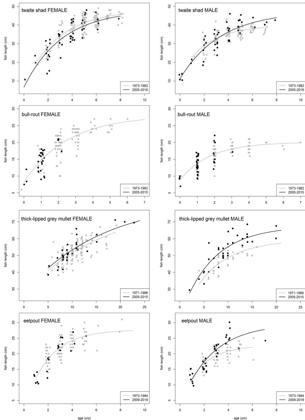
Fig. 5. Age-length relationships of female and male twaite shad, mullet, bull-rout and eelpout in the two periods. A combined fitted line is presented if the difference between periods was insignificant. The exact periods differed slightly between species depending on data availability.
