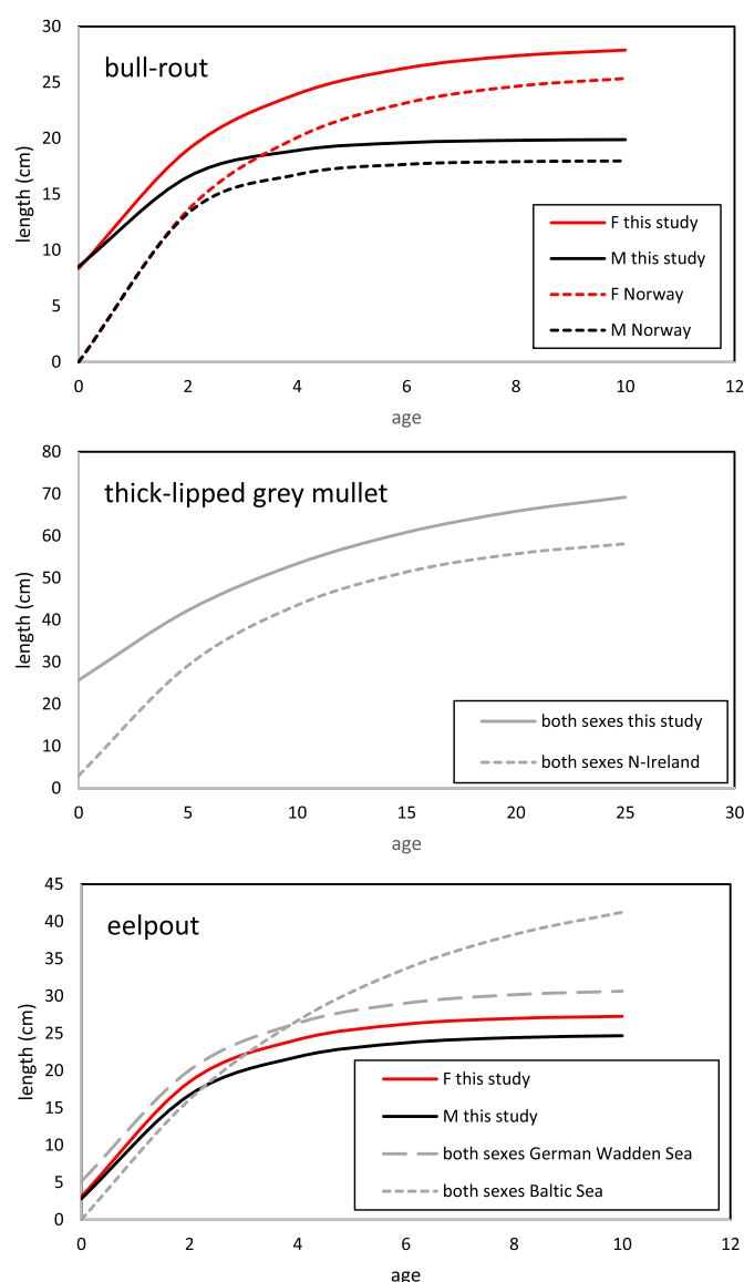
Fig. 8. Comparison of von Bertalanffy growth parameters with the literature (Luksenburg and Pedersen, 2002; Richter, 1995; Ulleweitt, 1995; Ulleweitt et al., 1998).
