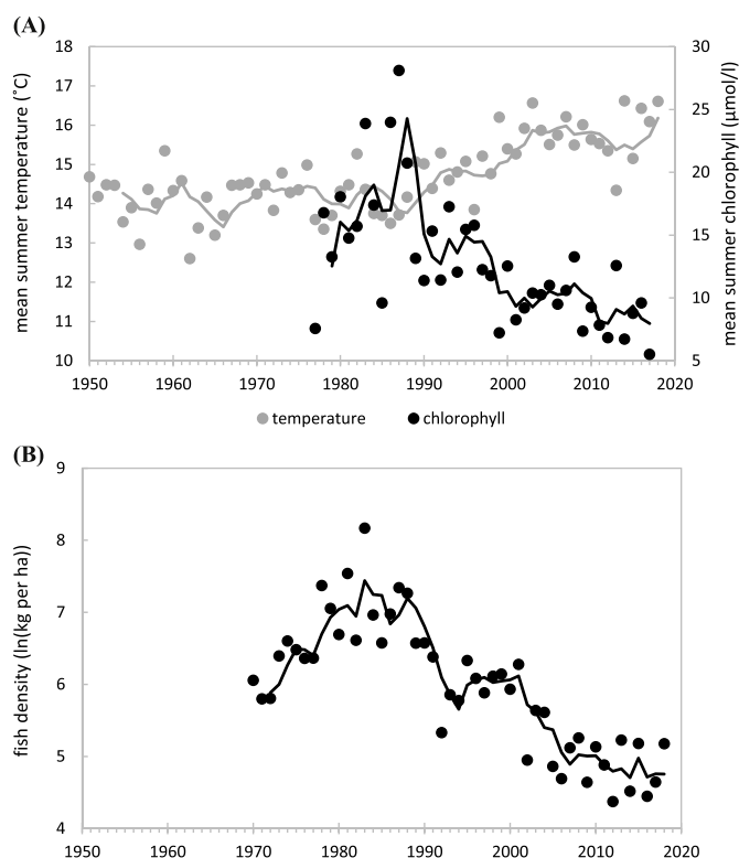
Fig. 2. (a) Long term trends of mean summer chlorophyll (May–Sept, from van Beusekom et al. (2017) ) and mean summer temperature (April–Sept, from van Aken (2008) ) in the Marsdiep. (b) Long term trends of fish density in the western Wadden Sea, based on the Demersal Fish Survey. Lines represent 3-year running means.
