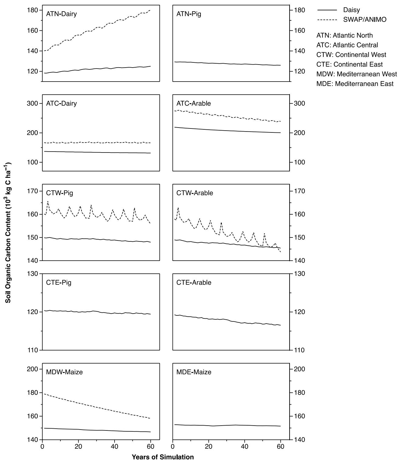
Figure 2.9: Soil organic C change in the logging depth over 60 years simulated by Daisy (solid line) and SWAP/ANIMO (dashed line). Changes were logged over the root zone, or 50 cm below the drain depth, whichever is deeper.
