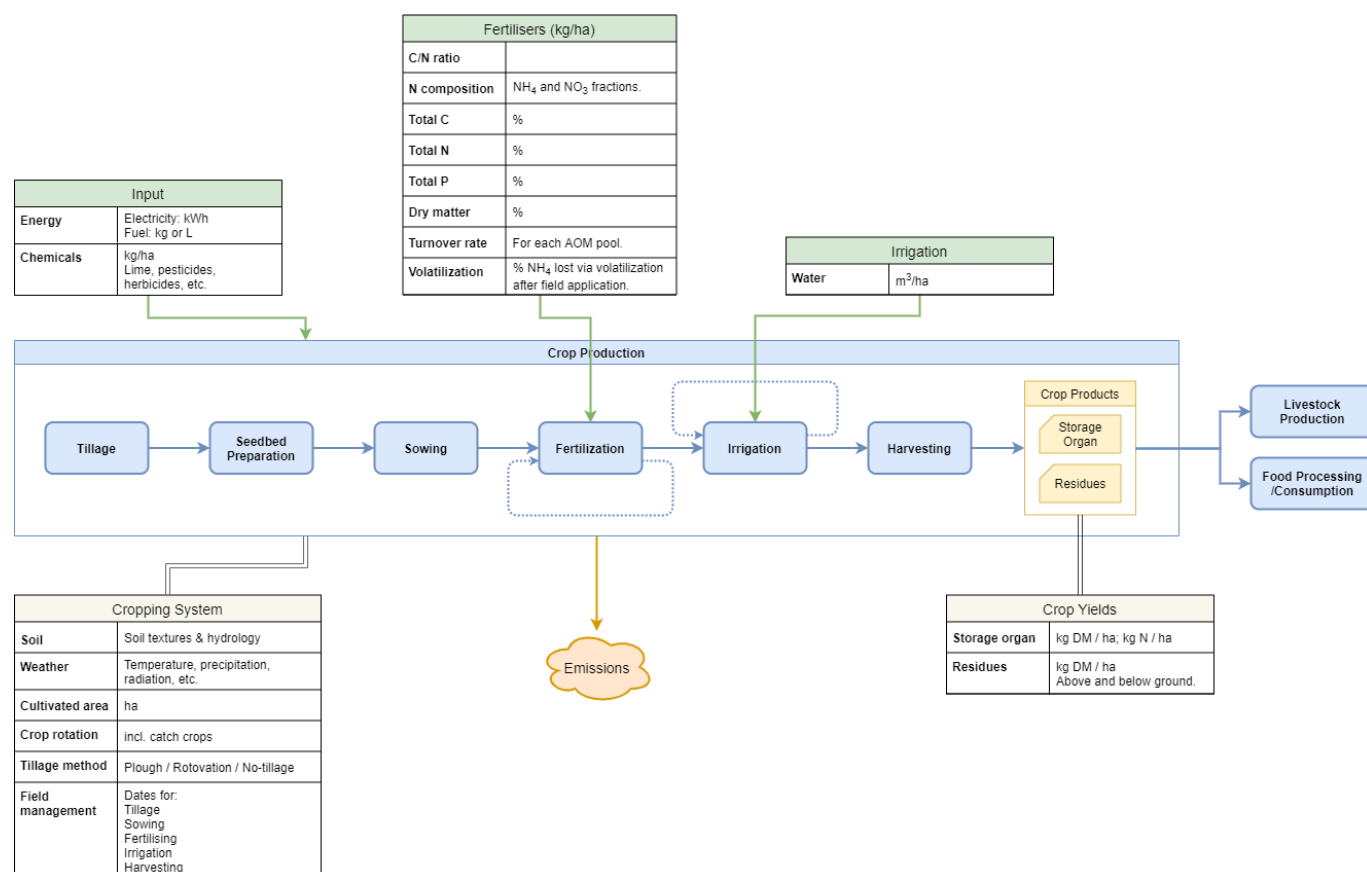
Figure 4.1: Schematic illustration of the processes and data requirement for the evaluation of environmental performances of novel fertilisers at field level.
