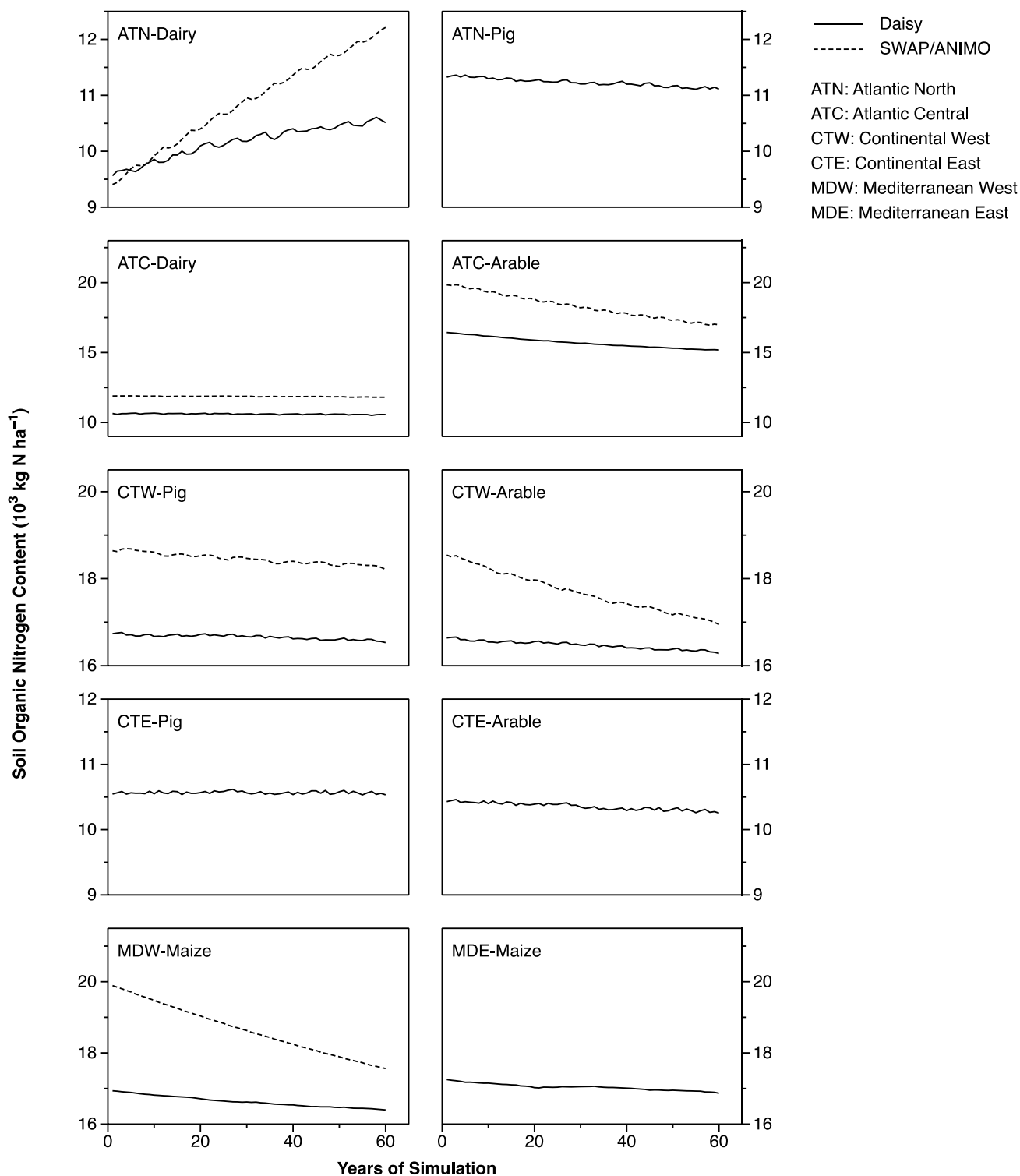
Figure 2.10: Soil organic N change in the logging depth over 60 years by simulated Daisy (solid line) and SWAP/ANIMO (dashed line). Changes were logged over the root zone, or 50 cm below the drain depth, whichever is deeper.
