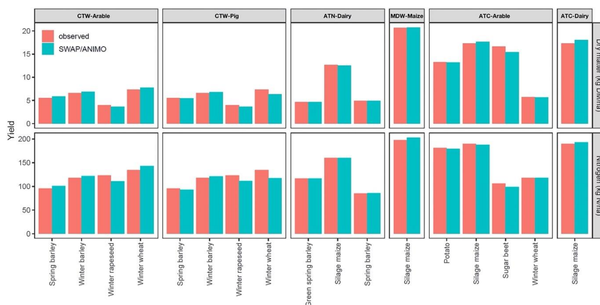
Figure 2.7: Crop dry matter (upper panels) and N yields (lower panels) of six selected scenarios, as simulated by SWAP/ANIMO (blue bars) and compared to observed yields (red bars).
