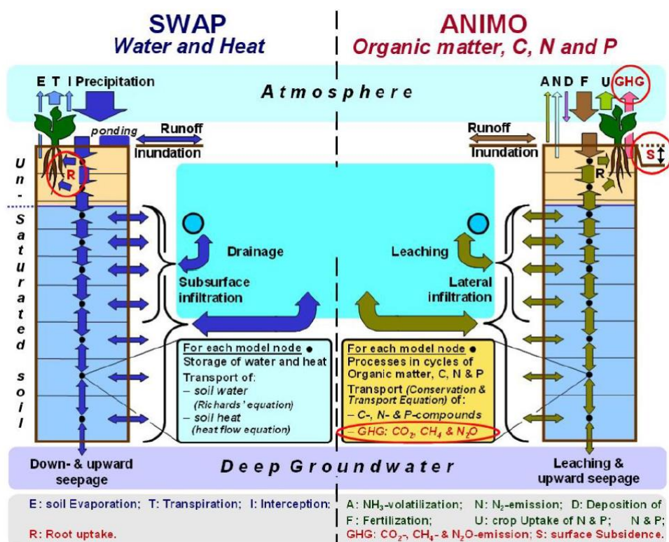
Figure 2.2: Schematic illustration of the SWAP/ANIMO models.
