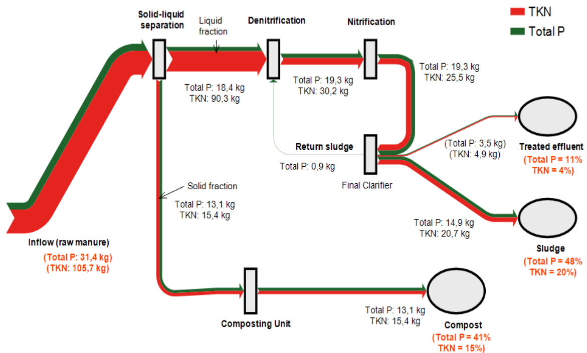
Figure 3.10 Illustration of TKN and P flows (in kg.day) from an NDN plant in Caldetenes, Spain (adapted from Foged et al. , 2011a).
