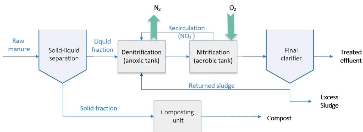
Figure 3.9 Process flow of a Nitrification-Denitrification system for N removal
