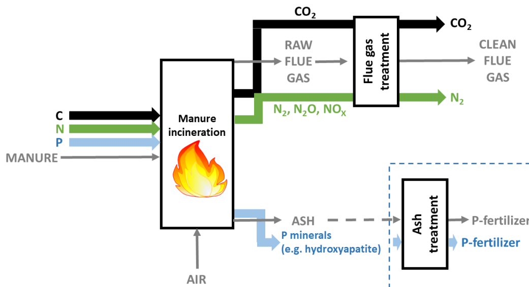
Figure 3.8 Simple schematic mass and elemental flow during manure incineration.
