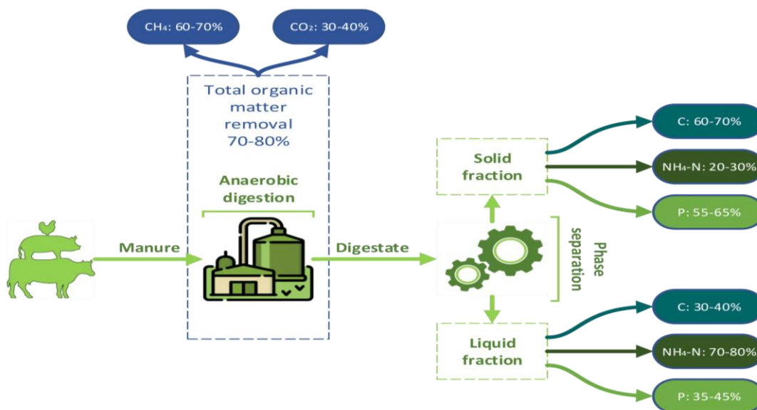
Figure 3.3 Schematic representation of CNP flows from digested manure
