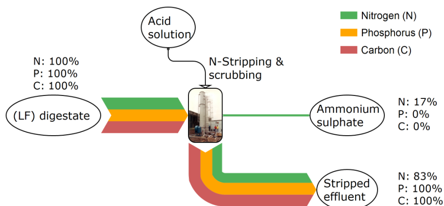
Figure 3.13 N, P and C fate during digestate processing by means of N-stripping, where 17% of total N is recuperated as ammonium sulphate solution. Adapted from Bolzonella et al. (2018).
