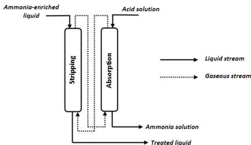
Figure 3.12 Schematic overview of the N-stripping process (Bernal et al. , 2015).
