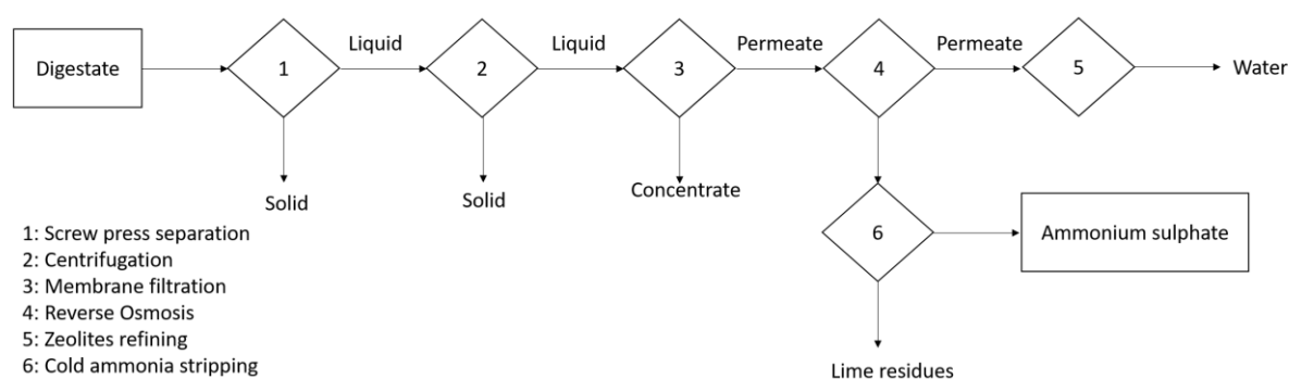
Figure 3.6 Six-step approach of the membrane plant (after Fangueiro et al., 2017)
