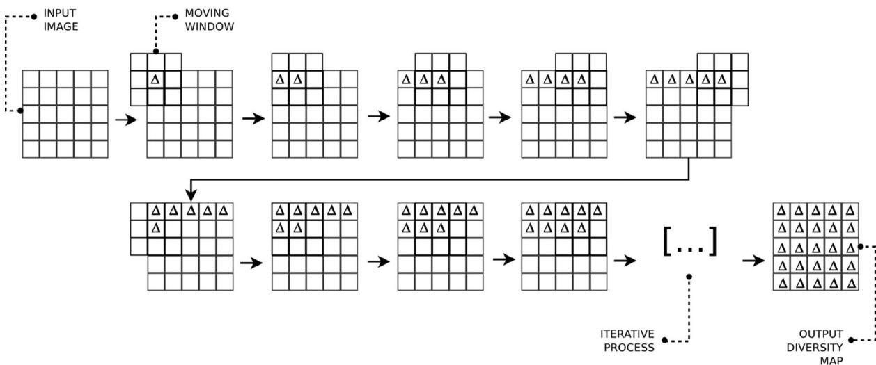
FIGURE 1 The moving window technique for the computation of diversity indices in the rasterdiv package, redrawn from Rocchini et al. (2013)
