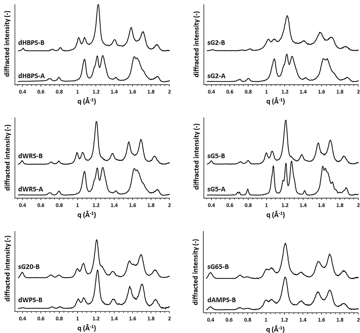
Fig. 2. XRD profiles of narrow and polydisperse RS-3 preparations.
