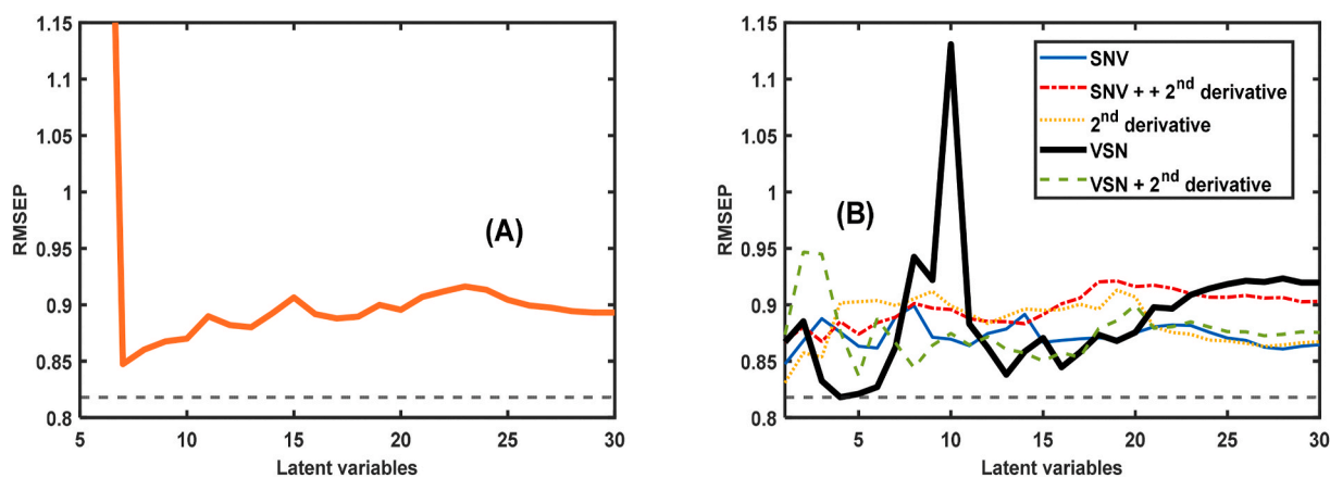
Fig. 7. (A) Evolution of RMSEP for PLS models for between 5 and 30 latent variables for raw absorbance data, and (B) evolution of RMSEP for differently pre-processed data, over the range of 1–30 latent variables, to find complementary information to the raw absorbance.
