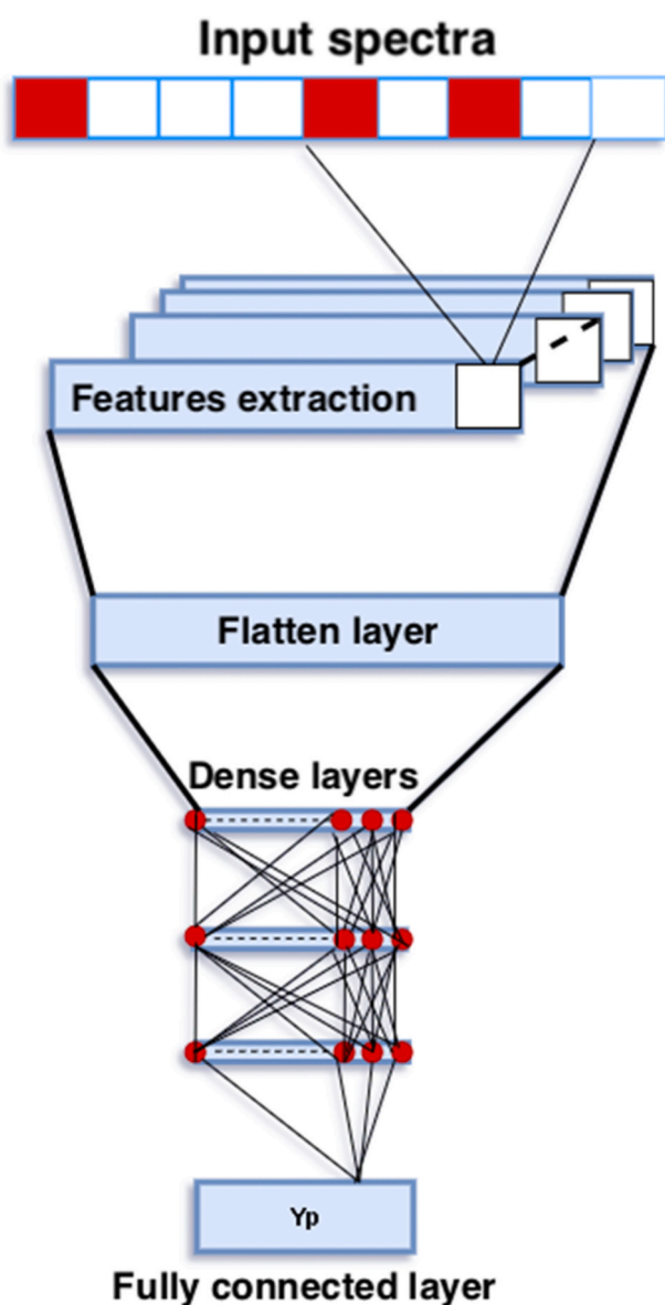
Fig. 1. A summary of the deep learning (DL) architecture implemented. The architecture consisted of one convolutional later and 3 dense fully connected layers.
