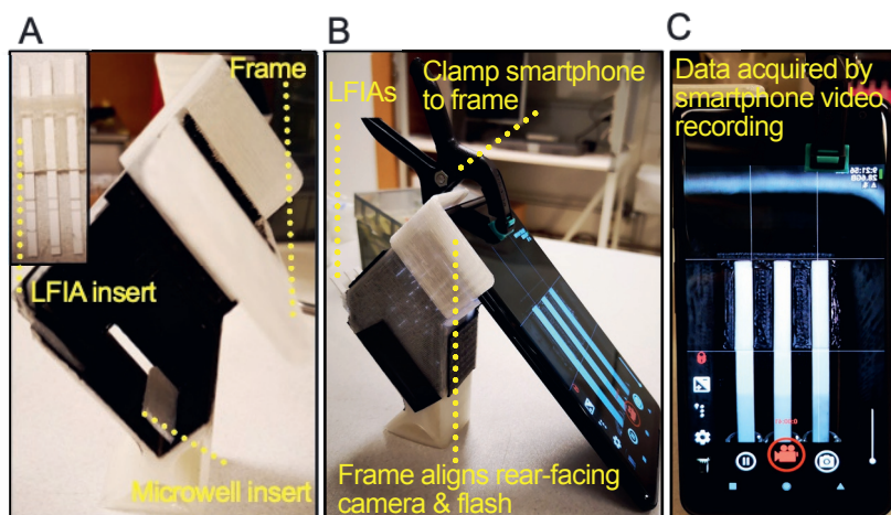
Figure 6.1. Photographs of the 3D-printed smartphone-holder for recording LFIA signal development under controlled lighting: (A) open side view to show where LFIAs and microwells are inserted; (B) closed side view with the LFIAs inserted and smartphone attached; (C) head-on view of LFIA signal development on the phone screen.
