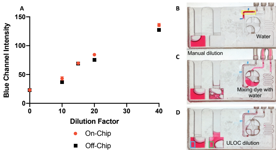
Figure 5.5. ULOC dilutor. (A) Graph depicting the performance of ULOC for unidirectional sample dilution as a function of blue channel intensity. The red circle represents ULOC dilutions. The black square represents manual dilutions. (B) ULOC before dilution, the area where the volume metering reading is taken from is outlined in yellow. (C) ULOC during dilution, the dye mixes with water in the reagent reservoir and is delivered to the test area by the fluidic system. (D) ULOC after dilution, intensity reading for the manual dilution (outlined in blue), and the intensity reading for the ULOC dilution (outlined in green).
