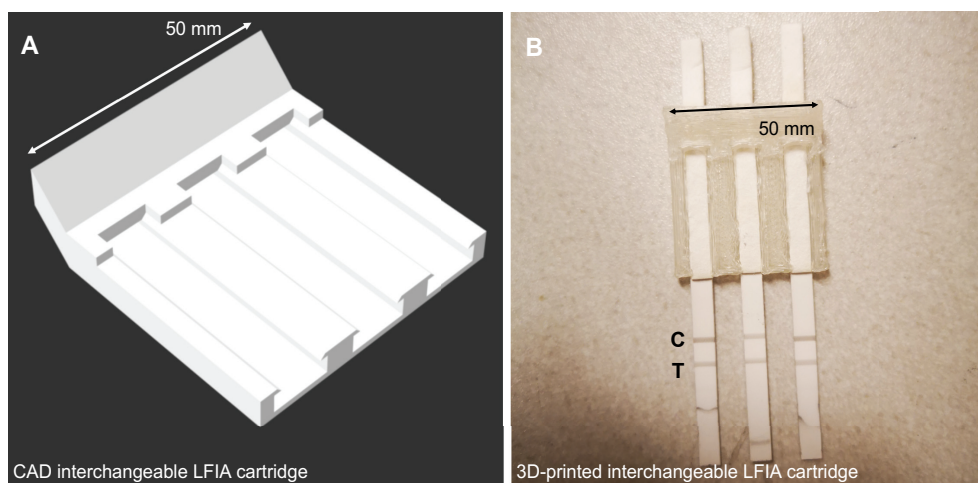
Figure S5.3. LFIA cartridge. (A) Computer aided design (CAD) of 50 mm LFIA cartridge which houses 3 LFIAs of 4 or 5 mm wide. (B) 3D-printed LFIA cartridge with 3 LFIAs inserted.
