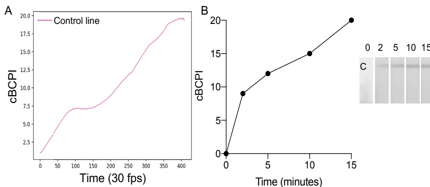
Figure S6.8. Dynamic monitoring of blank (0 ppm) LFIA signal development over 15 minutes. (A) Automatically generated binding profile where the pink line shows the control line, measurements are made every second (B) Manually plotted time-response profile and photographs showing control line development at 2, 5, 10 & 15 minutes.
