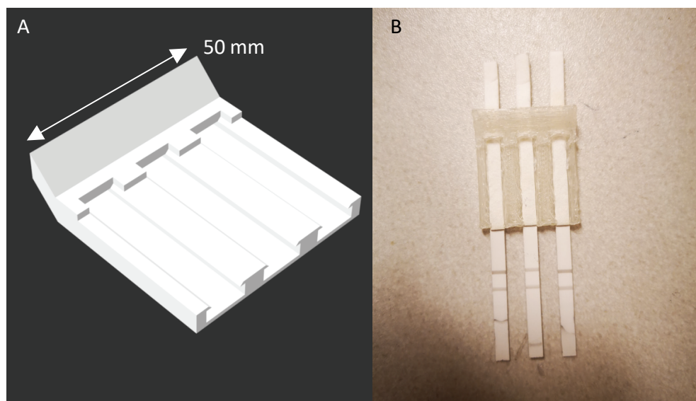
Figure S6.2. 3D-printed lateral flow immunoassay (LFIA) cartridge which allows 3 LFIAs to be recorded simultaneously. (A) computer aided design of the cartridge. (B) Photo of the 3D-printed LFIA cartridge, fitting 3 LFIAs.
