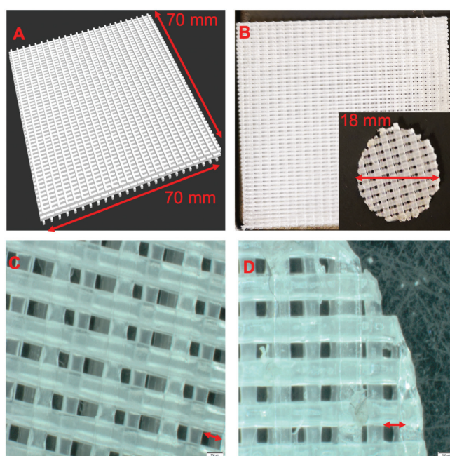
Figure S5.1. 3D-printed sieves. (A) Computer aided design (CAD) of sieve sheet. (B) 3D-print of the sieve sheet. Insert showing the 18 mm diameter laser cut sieves. (C) Microscope image of sieve, scale bar (500 \mu\text{m} ) in bottom right-hand corner and indicated by red arrow. (D) Microscope image of edge of laser cut sieve, scale bar (500 \mu\text{m} ) in bottom right-hand corner and indicated by red arrow.
