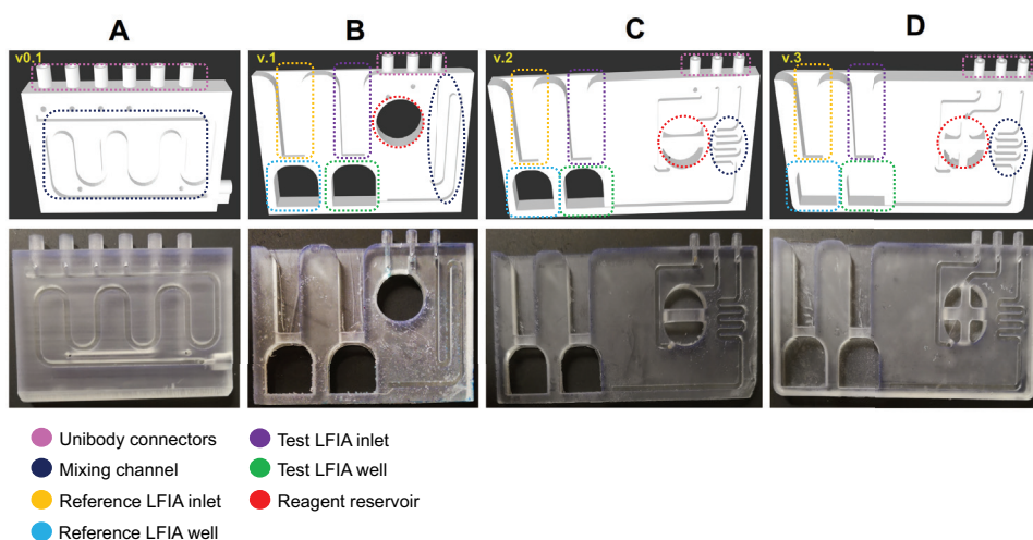
Figure 7.2. The design and development process for the ULOC dilutor showing the stl files and corresponding 3D-print; (A) the original design (v0.1), (B) the first design for integrating LFIA (v.1); (C) the improved design (v.2); (D) the penultimate structurally improved design (v.3).
