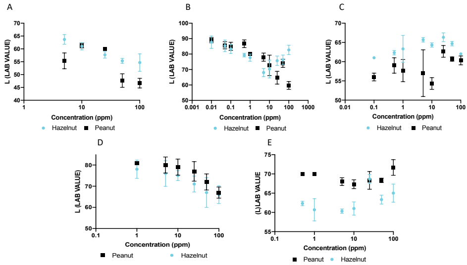
Figure S4.5. Calibration curves for smartphone analysis of lateral flow immunoassays using background subtraction. Smartphone (Huawei P20) analysis for lateral flow immunoassay Peanut Hazelnut Control (PHC) and Hazelnut Peanut Control (HPC) assays, plotted as a function of the concentration of Total Hazelnut Protein (THP) and Total Peanut Protein (TPP) spiked into Running Buffer (RB) (100–0.05 ppm). Where LAB values are obtained by subtraction of the background nitrocellulose values from the test lines. (A) PHC in 1 \mu L sample: 99 \mu L Running Buffer (RB) (B) PHC in 25 \mu L sample: 75 \mu L RB (C) PHC in 75 \mu L sample: 25 \mu L RB (D) HPC in 1 \mu L sample and 99 \mu L RB HPC in 25 \mu L sample: 75 \mu L RB. Error bars represent the standard deviation (n = 3).
