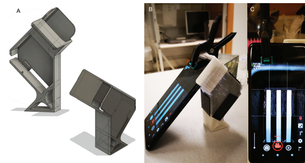
Figure S6.1. Smartphone holder for dynamic data acquisition of LFIA signal development. (A) Computer aided design of device holder. (B) Photograph of smartphone holder, with smartphone attached and real-time recording of 3 assays signal development. (C) Head on view of smartphone screen showing real-time signal development.
