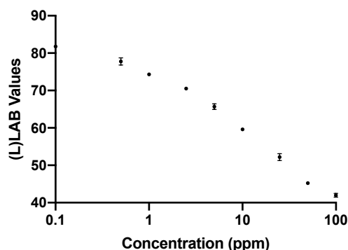
Figure 3.5. A calibration curve showing the relationship between (L)LAB values of test lines of hazelnut LFIA in a decreasing concentration of hazelnut protein (in blank cookie). Error bars have been included to show the standard deviation across multiple ( n = 3 ) measurements. An (L)LAB value of 100, (0, 0) corresponds to a true white and of 0 (0,0) to a true black, in this study the lowest L value was 42 and so the L (LAB) axis begins at 40.
