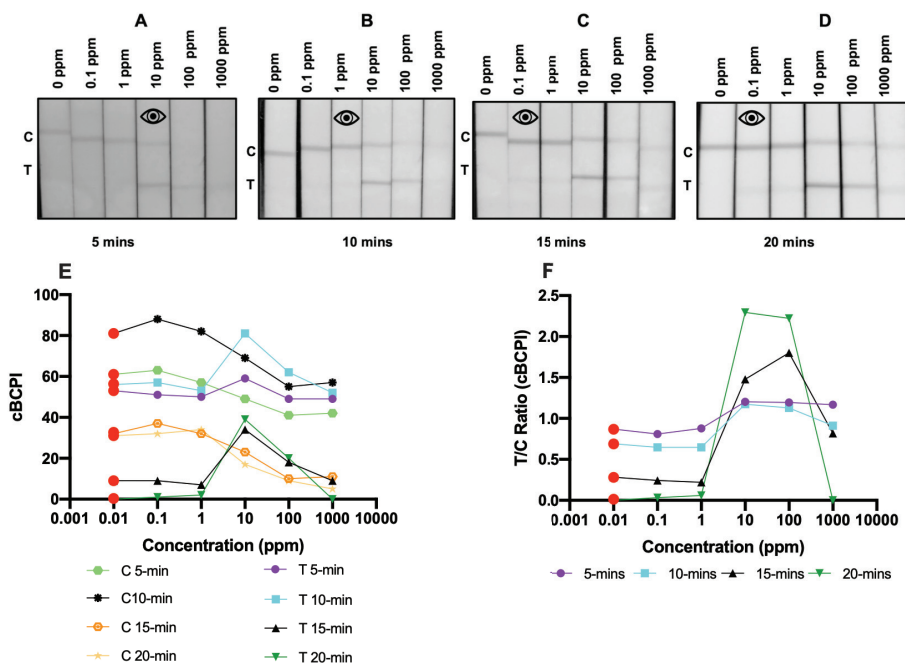
Figure S5.8. Endpoint images and calibration curves showing development of LFIs tested in an increasing concentration of total hazelnut protein (THP) extract in blank cookie (BC) extract in the range of 0.1-1000 ppm, C represents the control line and T represents the test line, the eye symbol represents the visual LOD at that given time point. All intensities are measured in the blue channel of RGB corrected by subtracting the background response of a blank test. (A) LFIs after 5 minutes. (B) LFIs after 10 minutes. (C) LFIs after 15 minutes. (D) LFIs after 20 minutes. (E) Calibration curve showing the corrected blue channel pixel intensity (cBCPI) response for the control (C) and test (T) line development (F) Calibration curve showing the test line divided by control line (T/C ratio) development.
