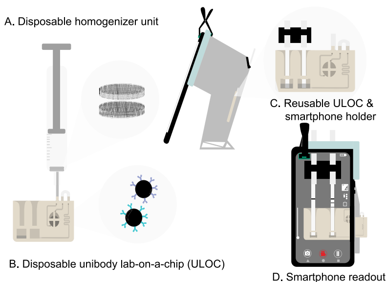
Figure 5.1. Overview schematic of parts of the prototype immunosensor. (A) Disposable homogenizer unit with 3D-printed sieves (B) Disposable unibody lab-on-a-chip (ULOC) for dilution of extracted allergens and mixing with carbon nanoparticle labeled allergen-specific antibodies. (C) Reusable smartphone and ULOC holder. (D) Smartphone readout, as a result, appears in real-time on the screen.
