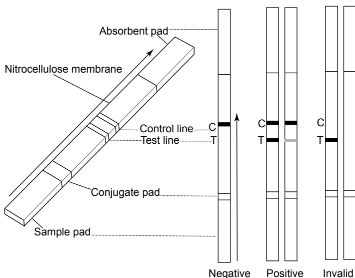
Figure 1.6. Schematic overview of the components in a typical singleplex LFIA and the possible results, where the arrows represent sample flow direction. (A) LFIA components: sample flows through the sample pad to the conjugate pad where any antigen in the sample interacts with labelled antibodies, the labeled antigen-analyte complex flows up the nitrocellulose membrane and is captured by the test line (T) and the control line (C), the absorbent pad acts as the fluid driving force for the LFIA. (B) LFIA tested in different sample types: C only means a sample is negative, C and T of any intensity means a sample is positive, only a T or no lines at all is indicative of an invalid sample concentration or LFIA.
