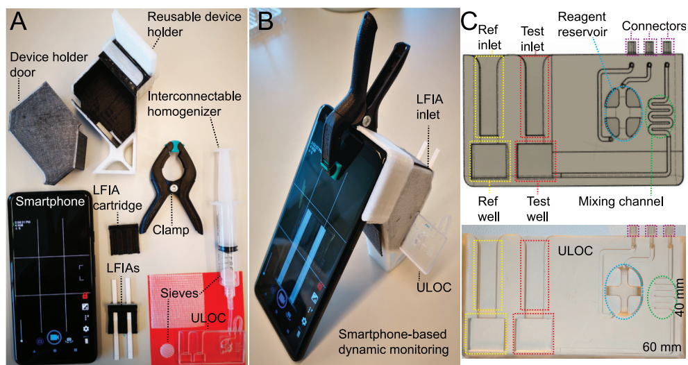
Figure 5.2. Overview of prototype immunosensor. (A) Disassembled prototype immunosensor showing all components. (B) Side view of the assembled device where the Unibody Lab on a Chip (ULOC) slots into the smartphone holder, the smartphone clamps to the holder's frame, the LFIAs insert into the opening, and the results are viewed on the phone. (C) Annotated Computer-Aided Design (CAD) and photo of the ULOC.
