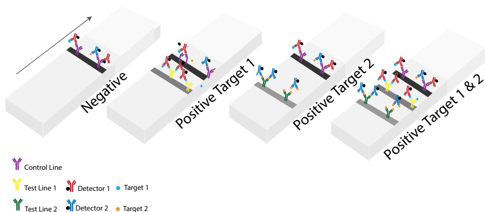
Figure 1.7. Schematic of multiplex lateral flow immunoassays (LFIAs) tested (left to right) in a negative sample, a sample positive for target 1, a sample positive for target 2, a sample positive for both targets. The arrow represents the flow direction.
