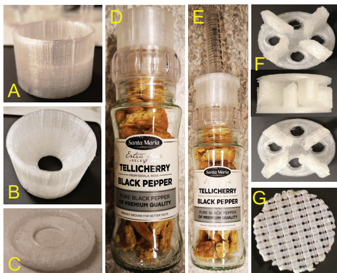
Figure 7.1. Developing the 3D-printed sample preparation unit; the body and lid of attachment (A-C), the pepper cracker with module attached (D) and syringe attached (E), the two-part grinder (F) the laser-cut sieves (G).
