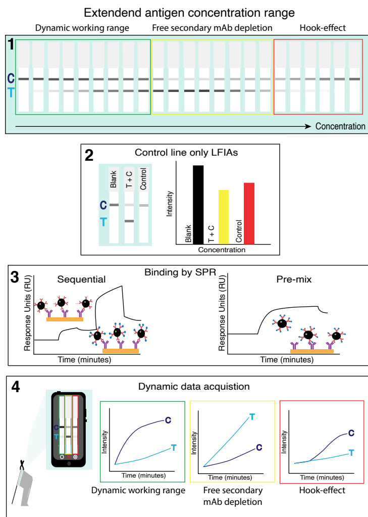
Figure S6.9. Schematic representation of the workflow of experiments for this study where the dynamic working ranges – green zone, free-secondary mAb depletion – yellow zone and hook-effect – red zone. First, lateral flow immunoassays (LFIA) are tested in an extended antigen concentration range. Next, LFIA in the yellow zone are tested in control line only experiments. After, the binding behaviors of the control antibody (purple) was tested using surface plasmon resonance (SPR), in sequential and pre-mix experiments. Finally, LFIA were dynamically monitored in the green, yellow and red zones to determine how their signal development is influenced by concentration, over time.
