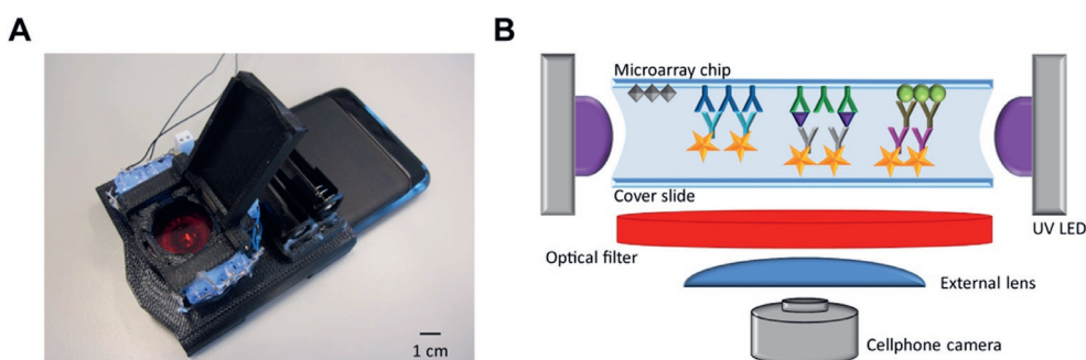
Figure 2.2. (A) Photo of 3D printed optical attachment on the smartphone used for testing. (B) Schematic representation of the smartphone biomarker detection platform. Reproduced with permission from authors (Ludwig et al. 2015).
