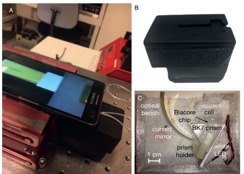
Figure 7.3. The smartphone-based prototype SPR platform; (A) photo of the SPR platform combined with a smartphone; (B) photo of the 3D-printed SPR platform (C) the inner components of the SPR platform. Photos credited to Xiao 2020.
