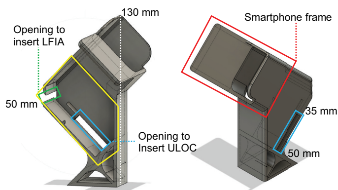
Figure S5.2. Computer aided design (CAD) image for smartphone device holder. Slot to insert ULOC is outlined in blue. The frame for clamping the smartphone to is outlined in red. The area to insert LFIA cartridge is outlined in green. The area which is closed by the door is outlined in yellow.
