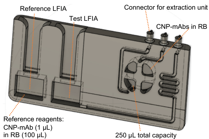
Figure S5.4. Annotated computer aided design (CAD) of the ULOC device indicating where the reference and test LFIAs are inserted, where the extraction unit connects to, where the carbon-nanoparticle labelled antibodies (CNP-mAbs) and running buffer (RB) are pre-loaded and where the reference reagents are pre-loaded.
