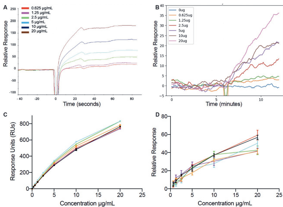
Figure 7.4. Performance comparison between a commercial Biacore 300 instrument and Xiao's smartphone-based prototype SPR-sensor. (A) Biacore: overlaid sensorgrams showing the detection of different concentrations of total hazelnut protein (THP) spiked in soymilk (0.625 – 20 µg/mL), (B) Prototype: overlaid sensorgrams showing the detection of different concentrations of total hazelnut protein (THP) spiked in soymilk (0.625 – 20 µg/mL), (C) Biacore: calibration curve showing the detection of a range of concentrations of THP in buffer and different plant-based milks as a function of RU. Error bars represent standard deviation (n=3). (D) Prototype: calibration curve showing the detection of a range of concentrations of THP in buffer and different plant-based milks as a function of relative response. Error bars represent standard deviation (n=3).
