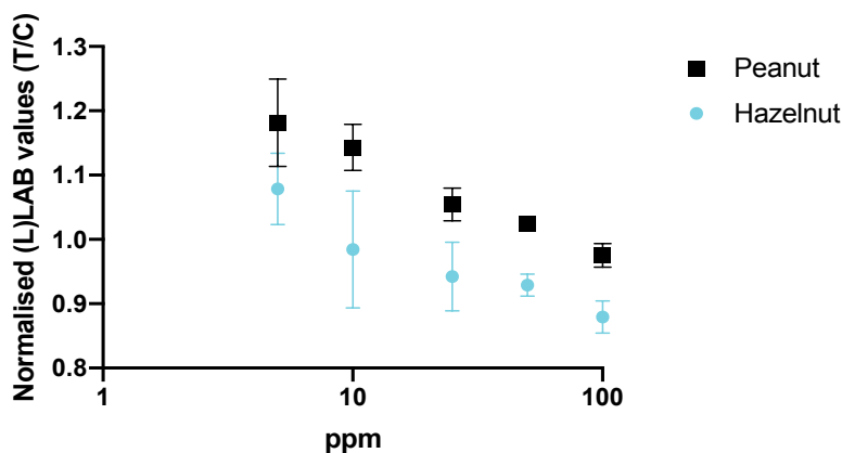
Figure S4.4. Calibration range for smartphone analysis of hazelnut, peanut, control (HPC) lateral flow immunoassay. Smartphone (Huawei P20) analysis, where normalized L (LAB) values (test line intensity/control line intensity; T/C) are plotted as a function of the concentration (100–5 ppm) Total Hazelnut Protein (THP) and Total Peanut Protein (TPP) spiked into Running Buffer (RB) (1 \mu L of the given dilution was diluted in 99 \mu L of RB). Error bars represent the standard deviation (n = 3). For experimental details, see the full manuscript.
