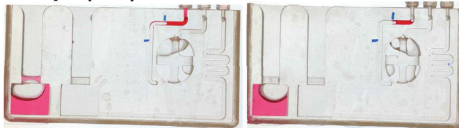
Figure S5.5. Unibody Lab on a Chip (ULOC) devices showing loading of dye to (A) 10 \mu L mark (n=2) (B) 5 \mu L mark (n=2).
