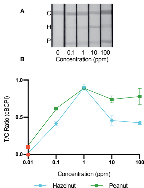
Figure 5.7. Photographs and calibration curves showing multiplex LFIA signal development in increasing concentration of incurred multi-allergen analyte where error bars represent standard deviation ( n=3 ). (A) Multiplex calibration range for sample type D2 (i.e., hazelnut cookie and peanut cookie spiked into blank cookie 0.1–100 ppm (w/w)) where C denotes the control line, H the hazelnut test line and P the peanut test line. (B) Calibration curve as a function of the T/C ratio (i.e., test line intensity divided by control line intensity) using corrected blue channel pixel intensities. The red circle represents the T/C ratio in a blank (0 ppm) sample.
