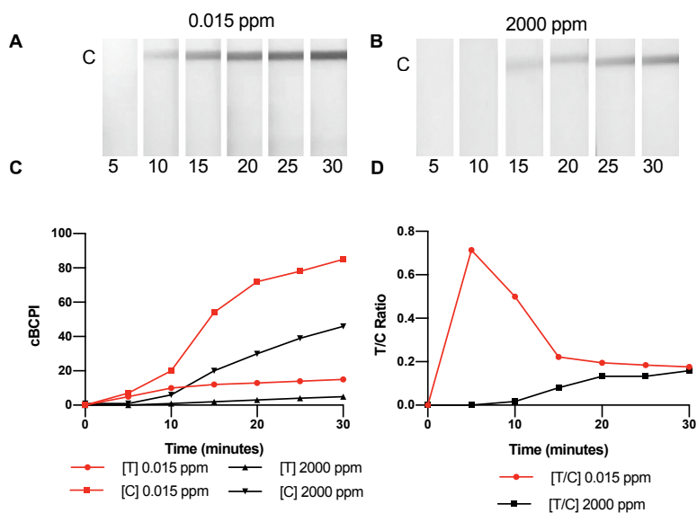
Figure S6.6. LFIA signal development over 30 minutes at 5-minute intervals in concentrations of (A) 0.015 ppm & (B) 2000 ppm of total hazelnut protein (C) the corrected blue channel pixel intensity (cBCPI) of test T and control C development at 0.015 ppm (red) and the C and T development (black). (D) the T/C development at 0.015 ppm and 2000 ppm.
