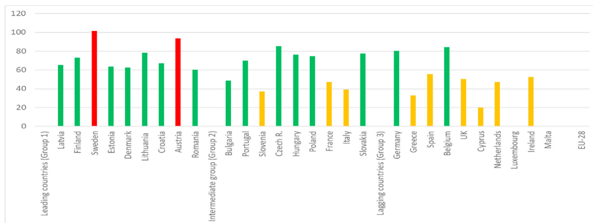
Fig. 7. Felling as percent of net annual increment in 2010 in FAWS [80,84]. Legend: Red bars >90% of NAI is harvested; green bars; up to 90% of NAI harvested, regarded as sustainable [83]; orange bars; underutilized harvest < 60%.
